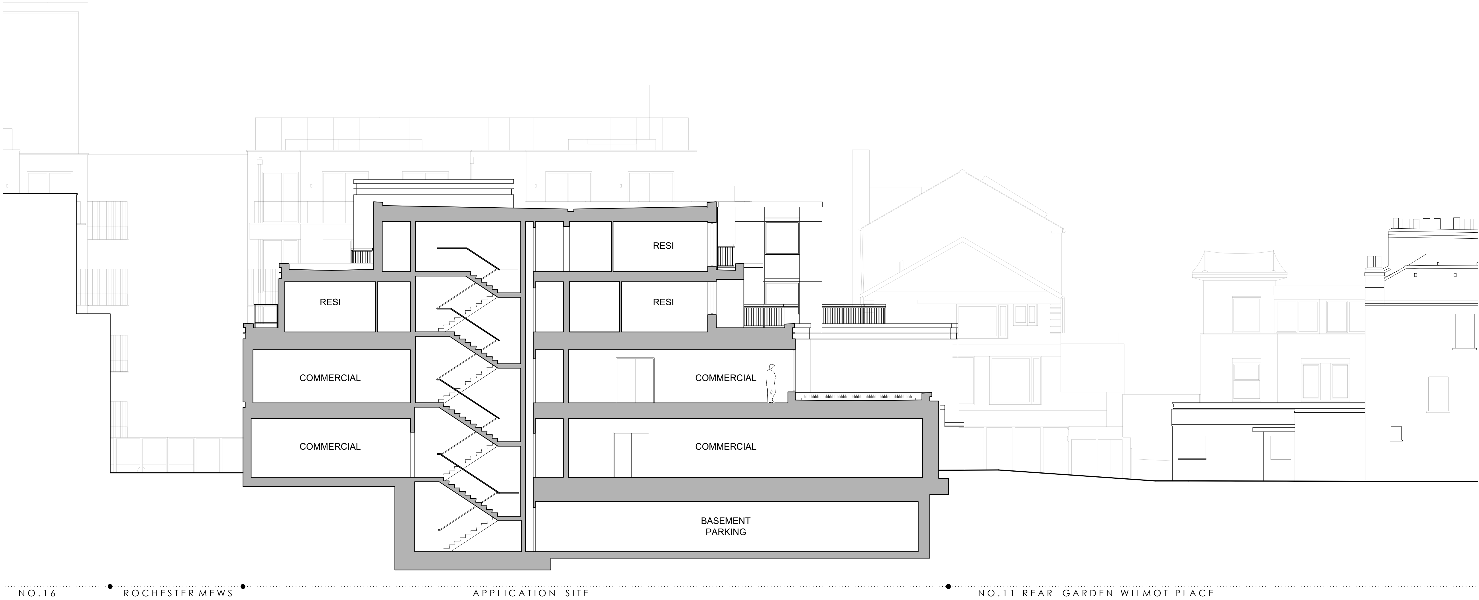
SECTION AA
