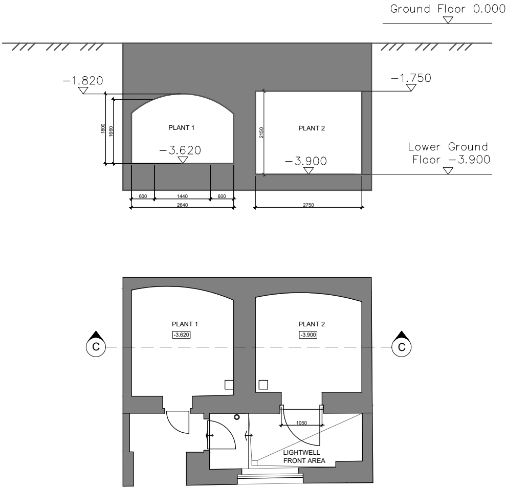
Existing Section C-C
