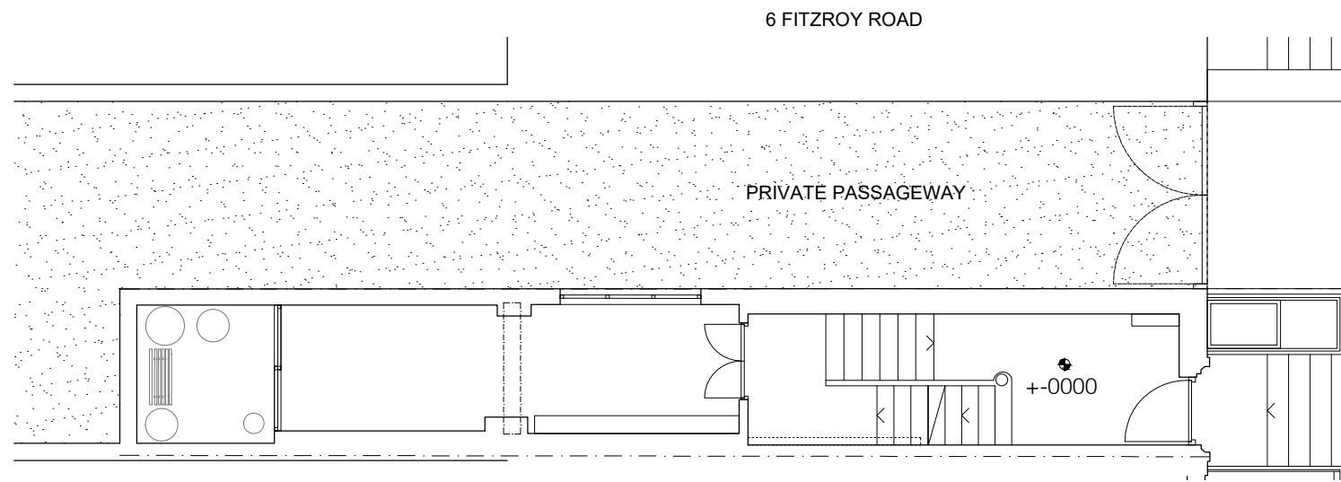
217-(00)100.02 - GROUND FLOOR PLAN
