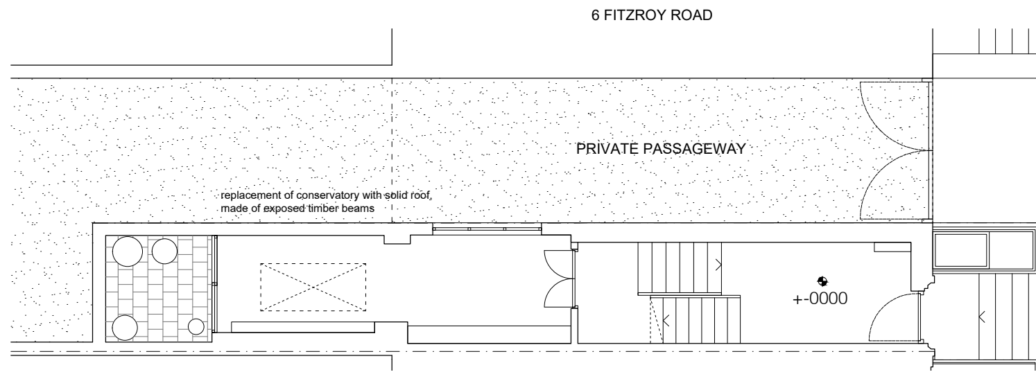
217-(01)100.02 - GROUND FLOOR PLAN
