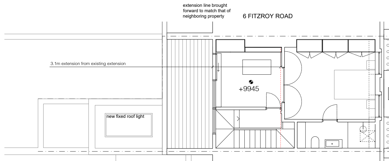
217-(01)100.02 - THIRD FLOOR PLAN
