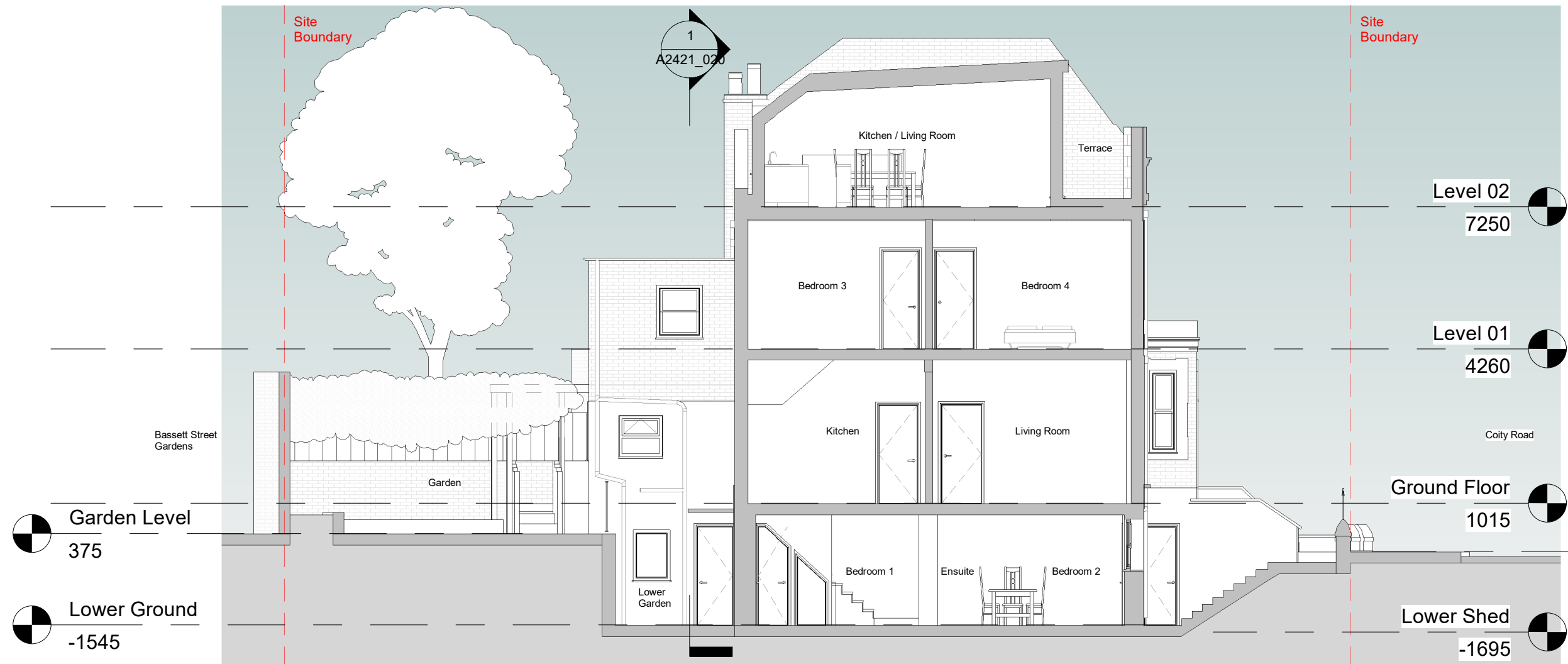
Proposed Section B-B
