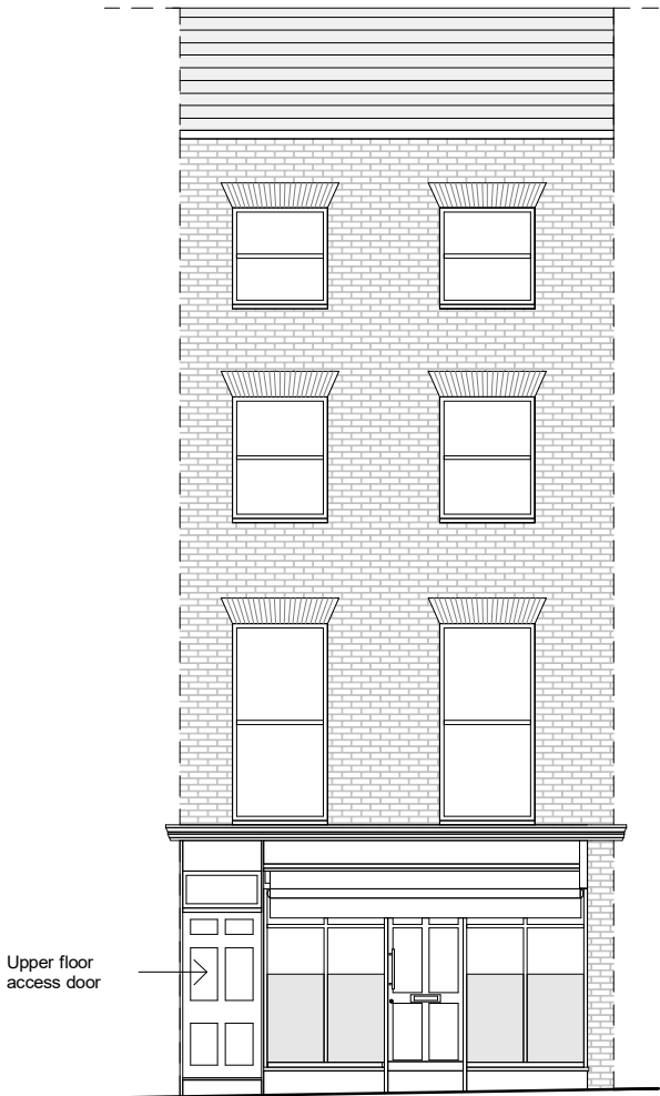
1 Existing Front Elevation 1 : 100
