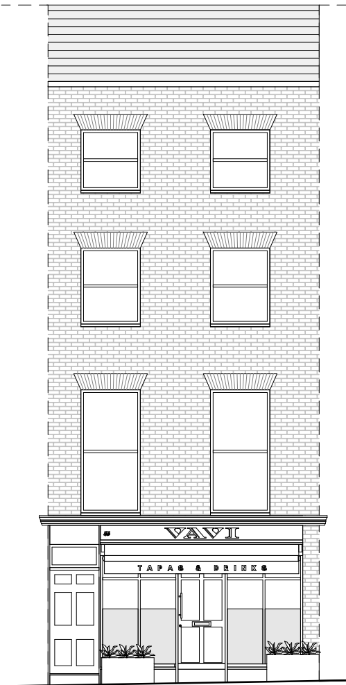
2 Proposed Front Elevation 1 : 100
