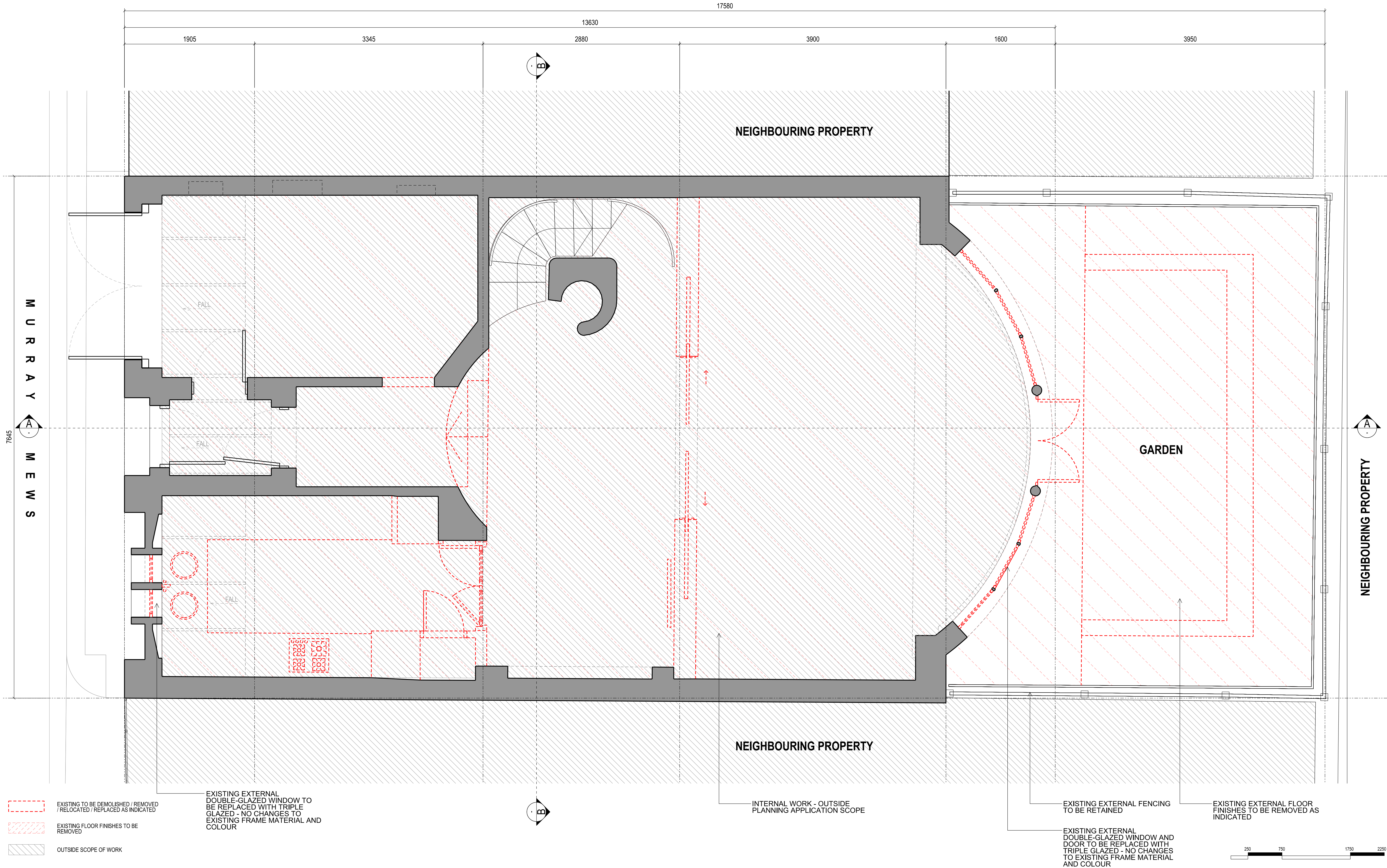
1 EXISTING GROUND FLOOR - DEMOLITION PLAN Scale 1:50 at A3 / 1:25 at A1
