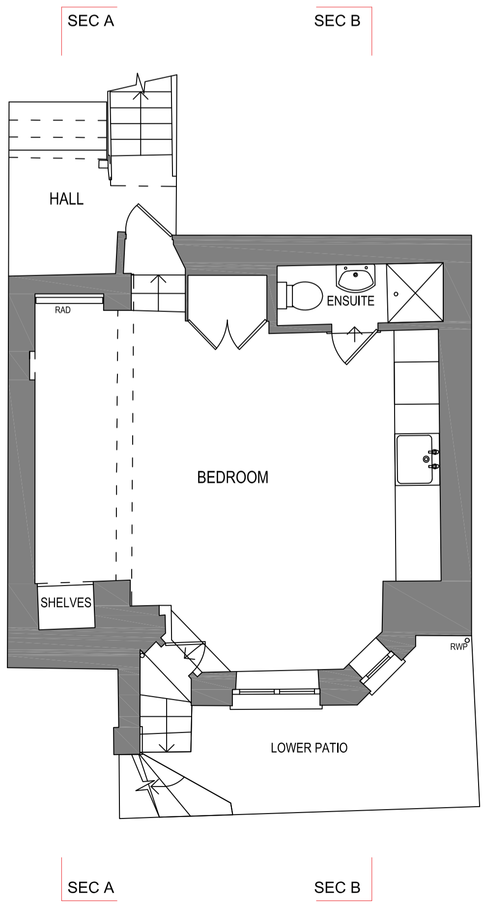
EXISTING LOWER GROUND FLOOR
