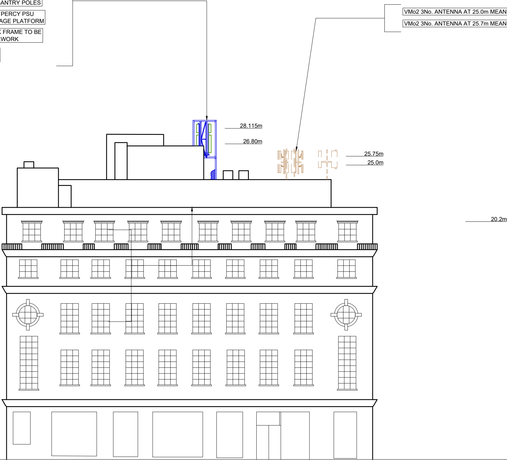
NORTH EAST ELEVATION SCALE 1:200
