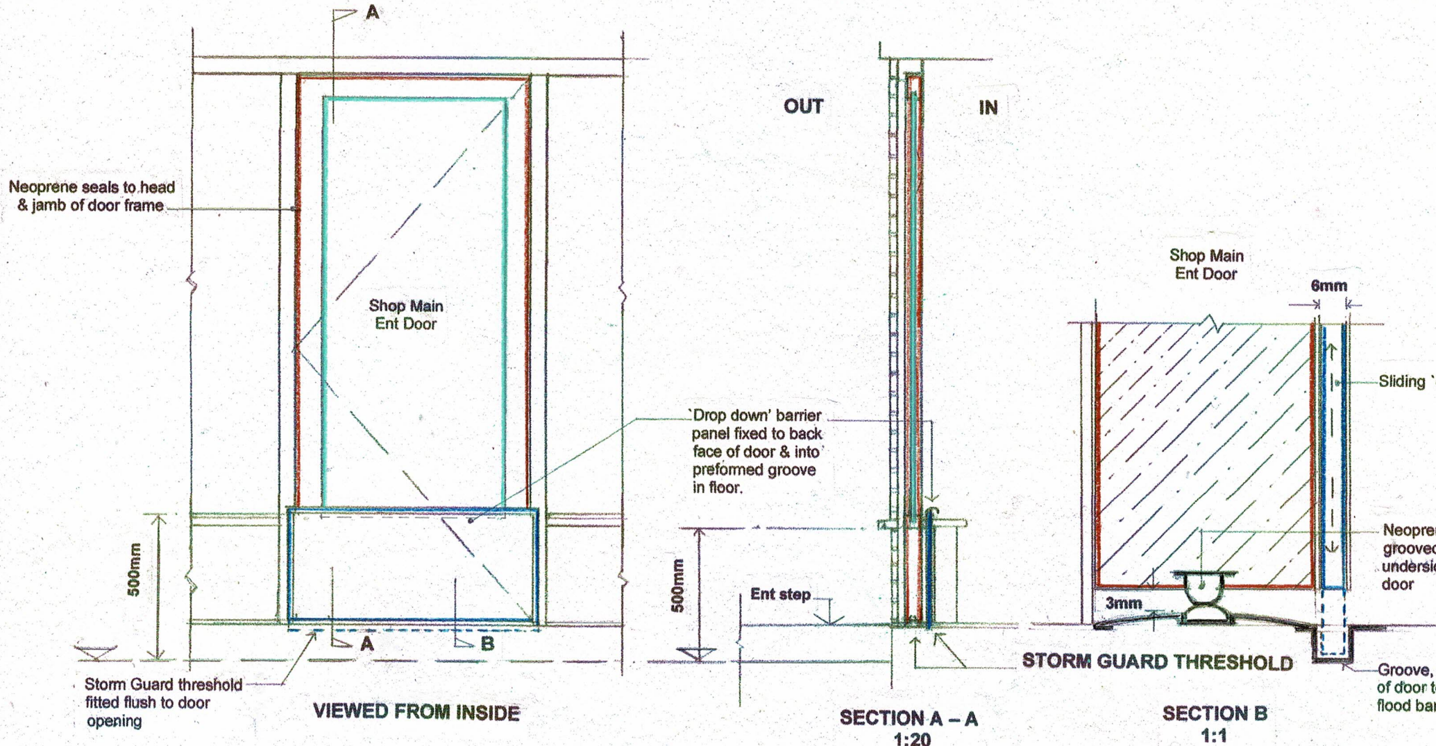
DROP DOWN FLOOR BARRIER DETAIL TO MAIN
