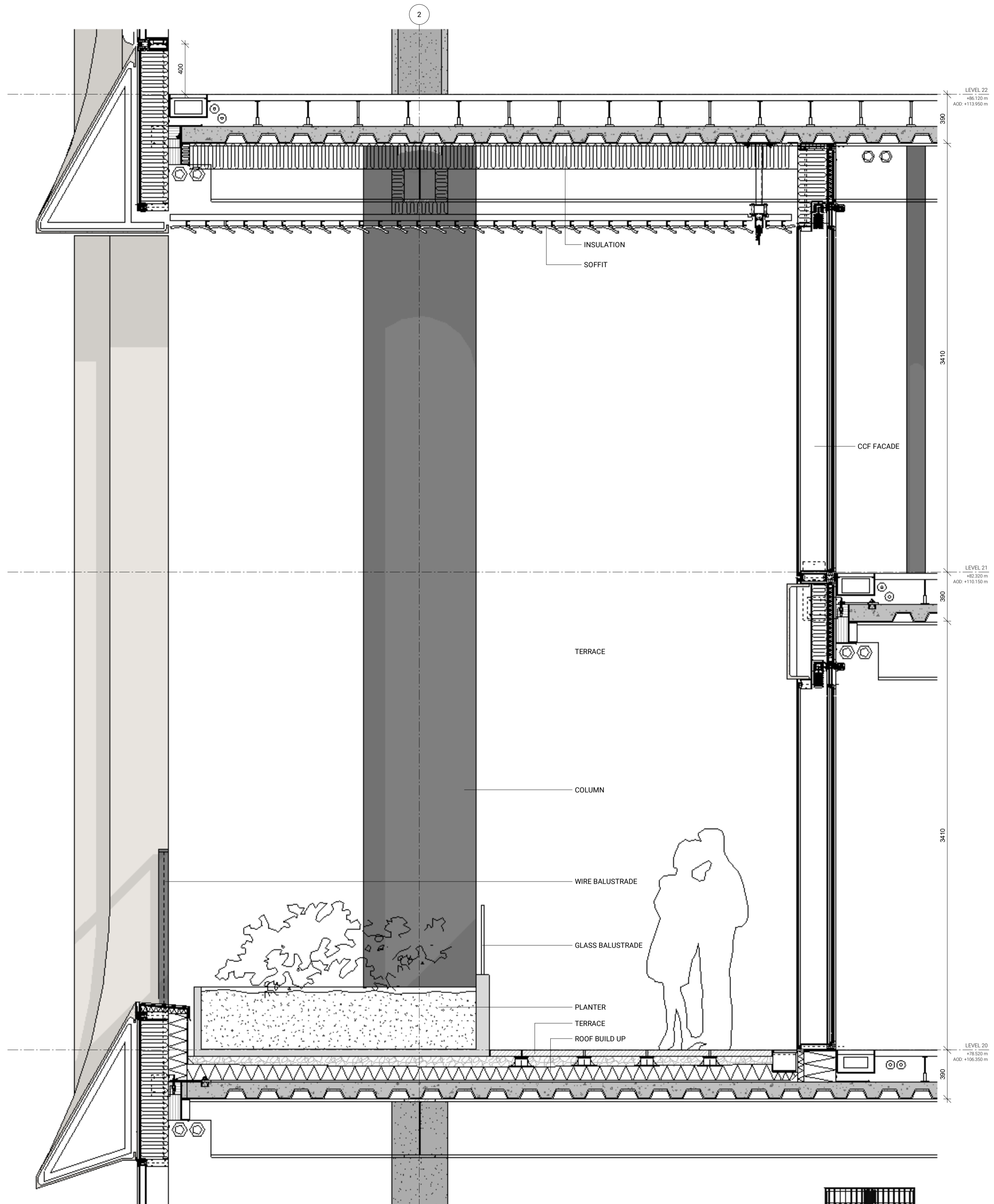
SECTION 1 1:20
