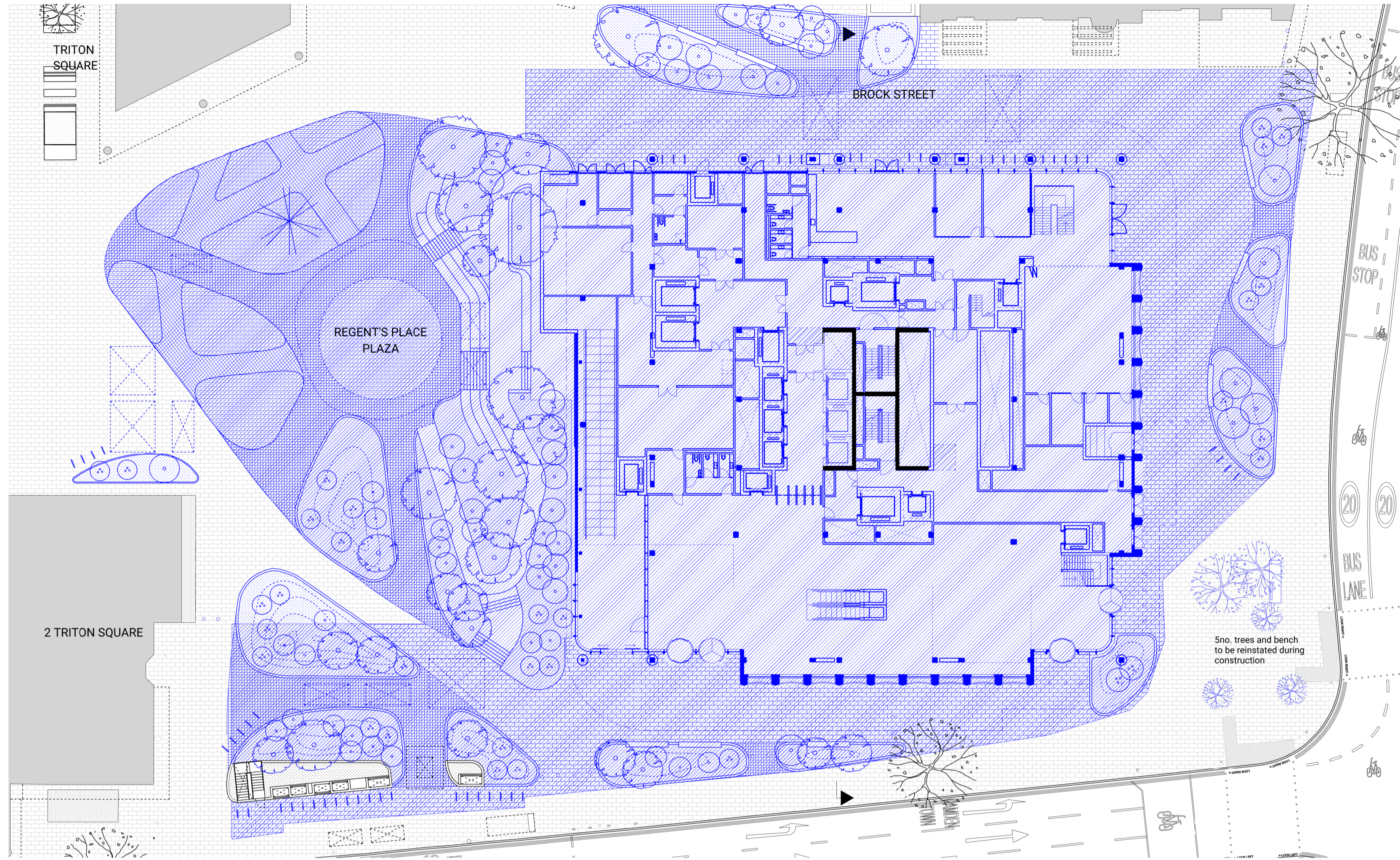
1 Phase 1 - Construction Plan - Ground Floor 1:300 @ A1
