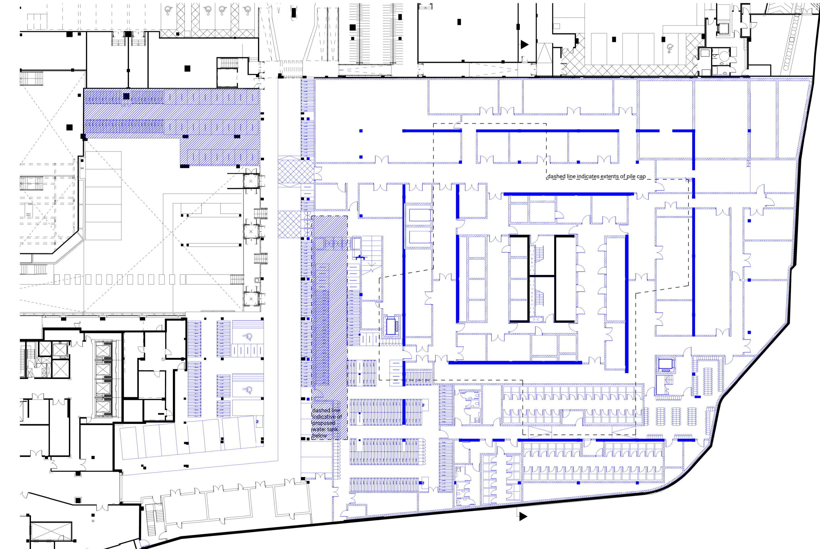
2 Phase 1 - Construction Plan - Basement 1:300 @ A1
