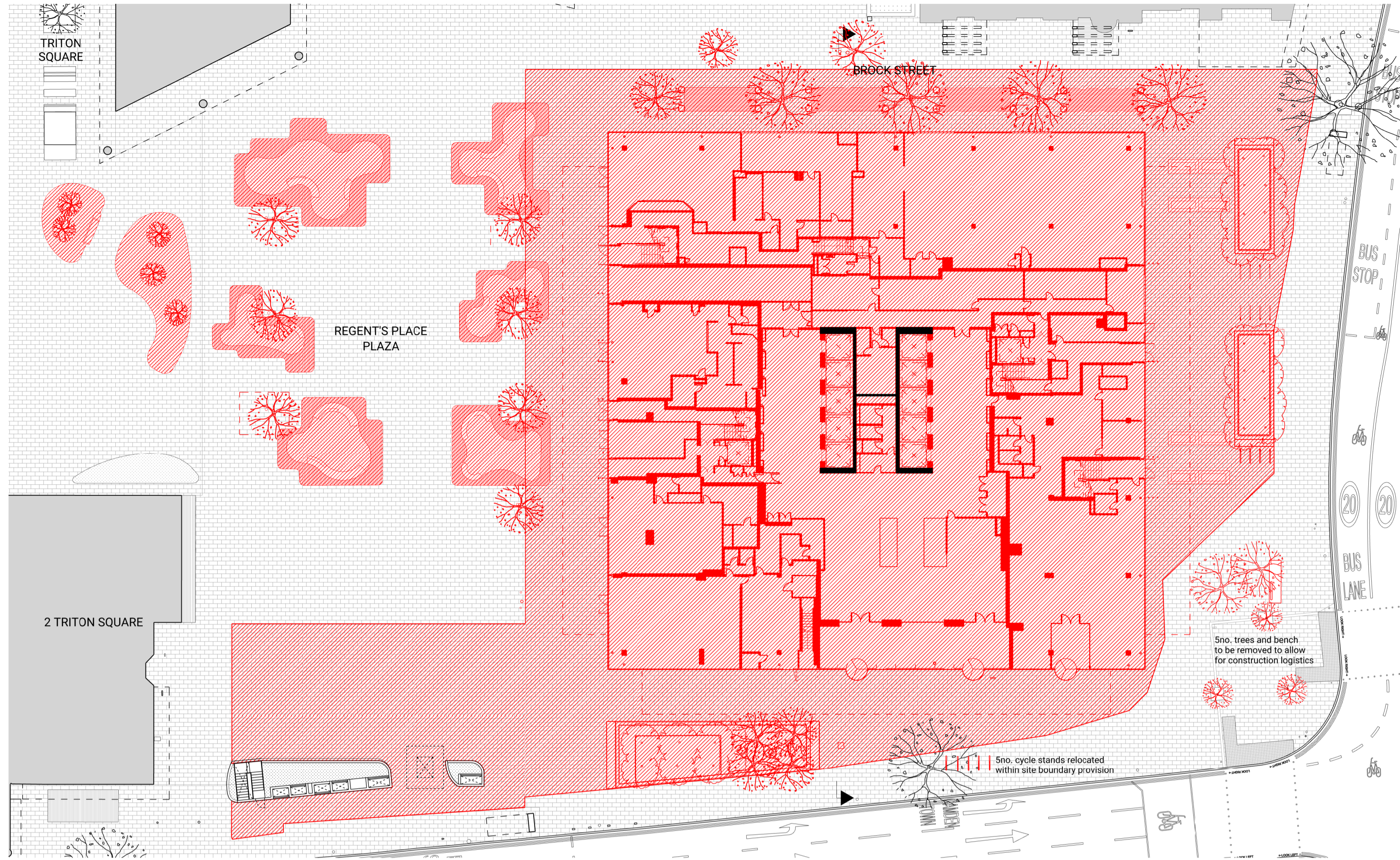
1 Phase 1 - Deconstruction Plan - Ground Floor 1:300 @ A1
