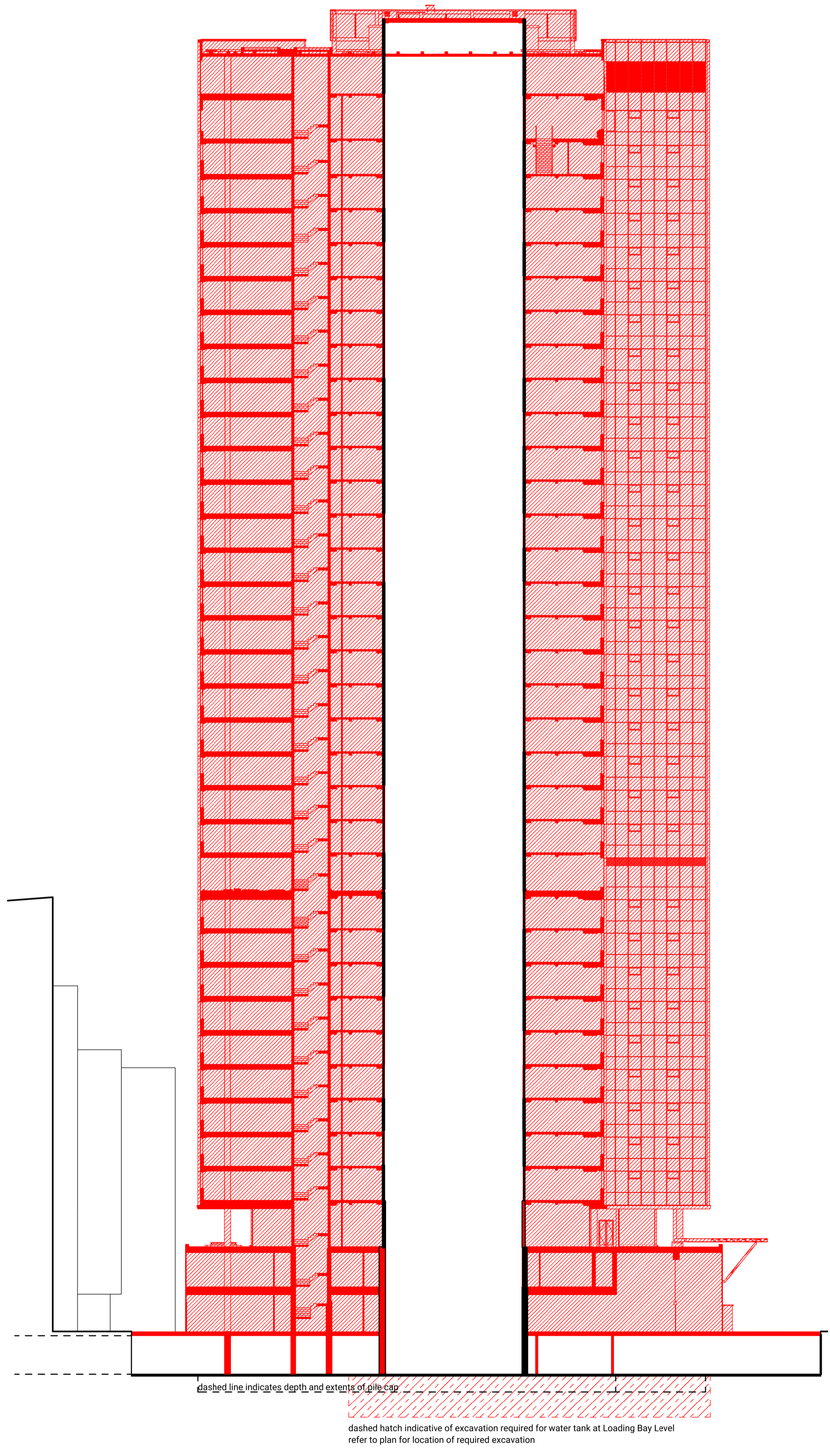
3 Phase 1 - Deconstruction Section 1:300 @ A1
