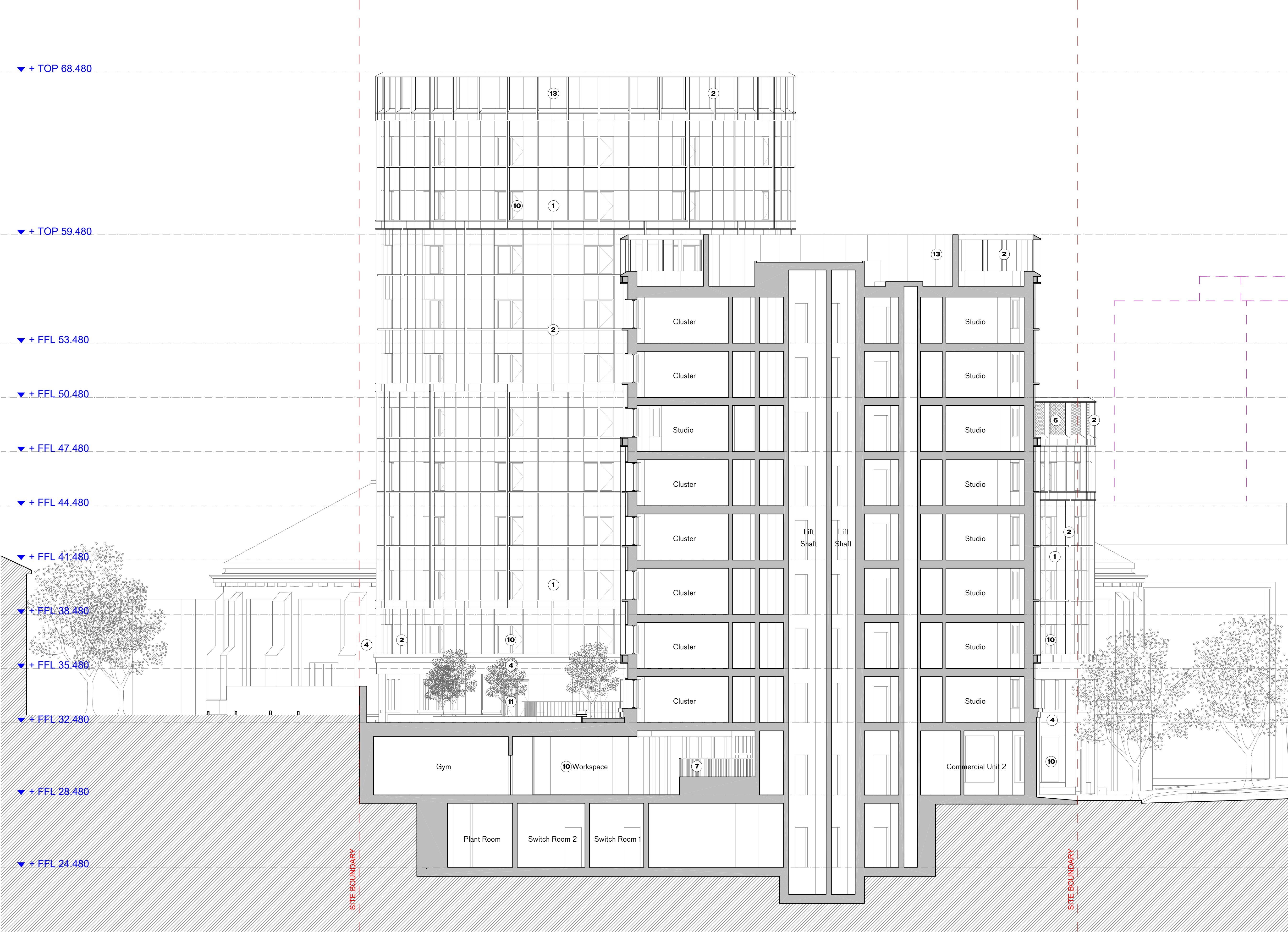
PBSA Building Section CC
