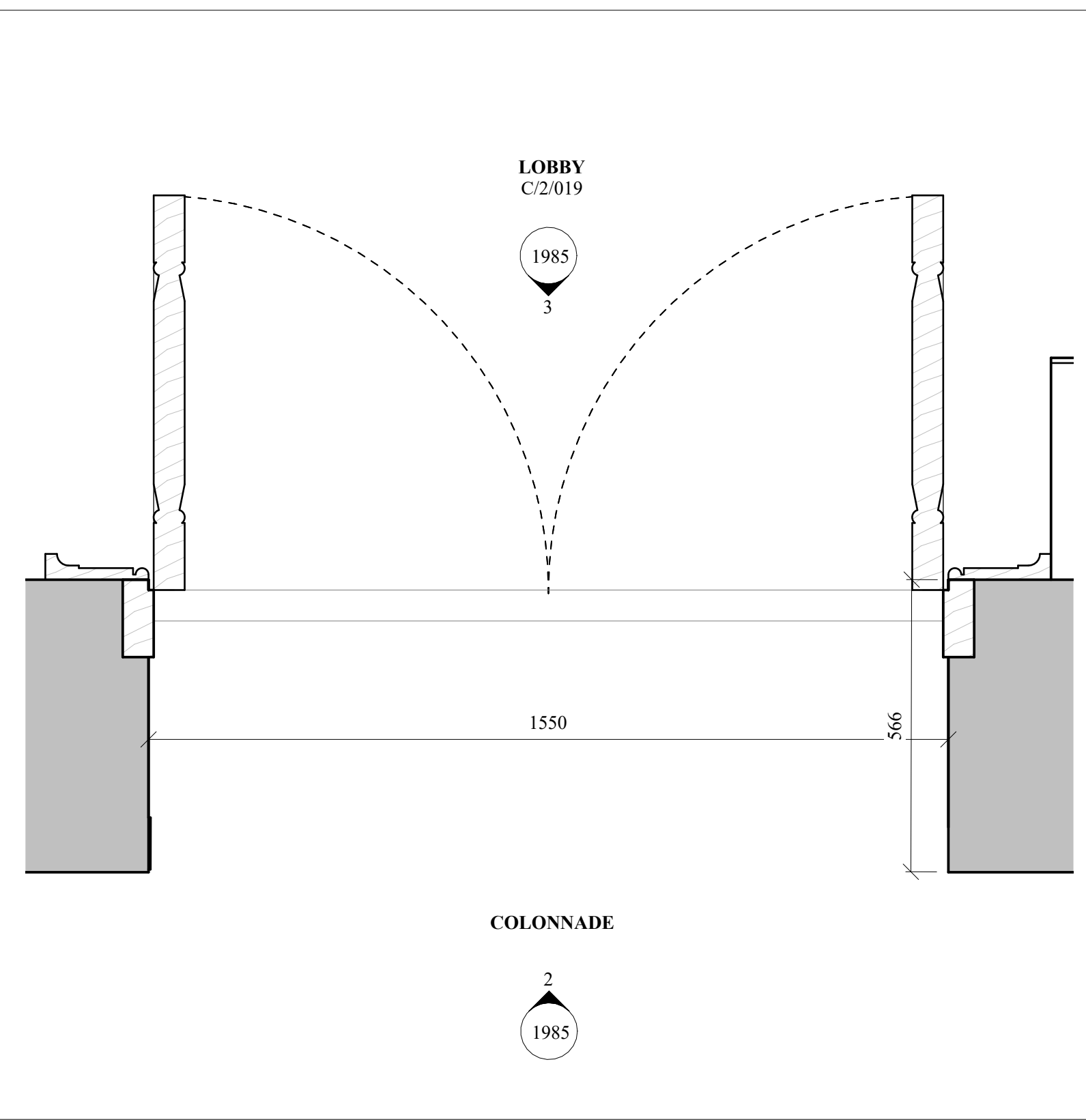
1 Level 2 South-West Wing External Door Plan
