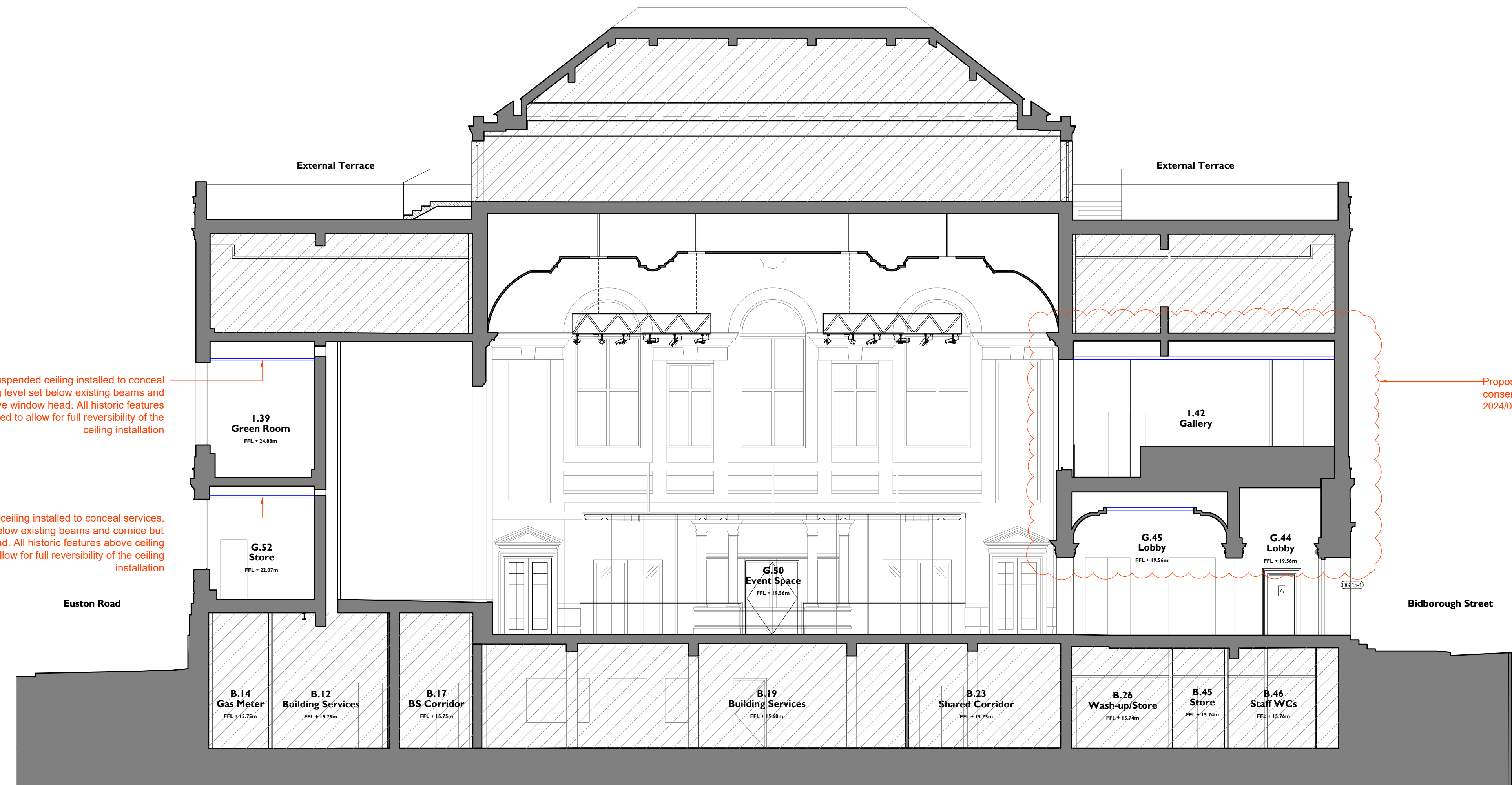
02 SECTION A-A - PROPOSED 0020 1:200
