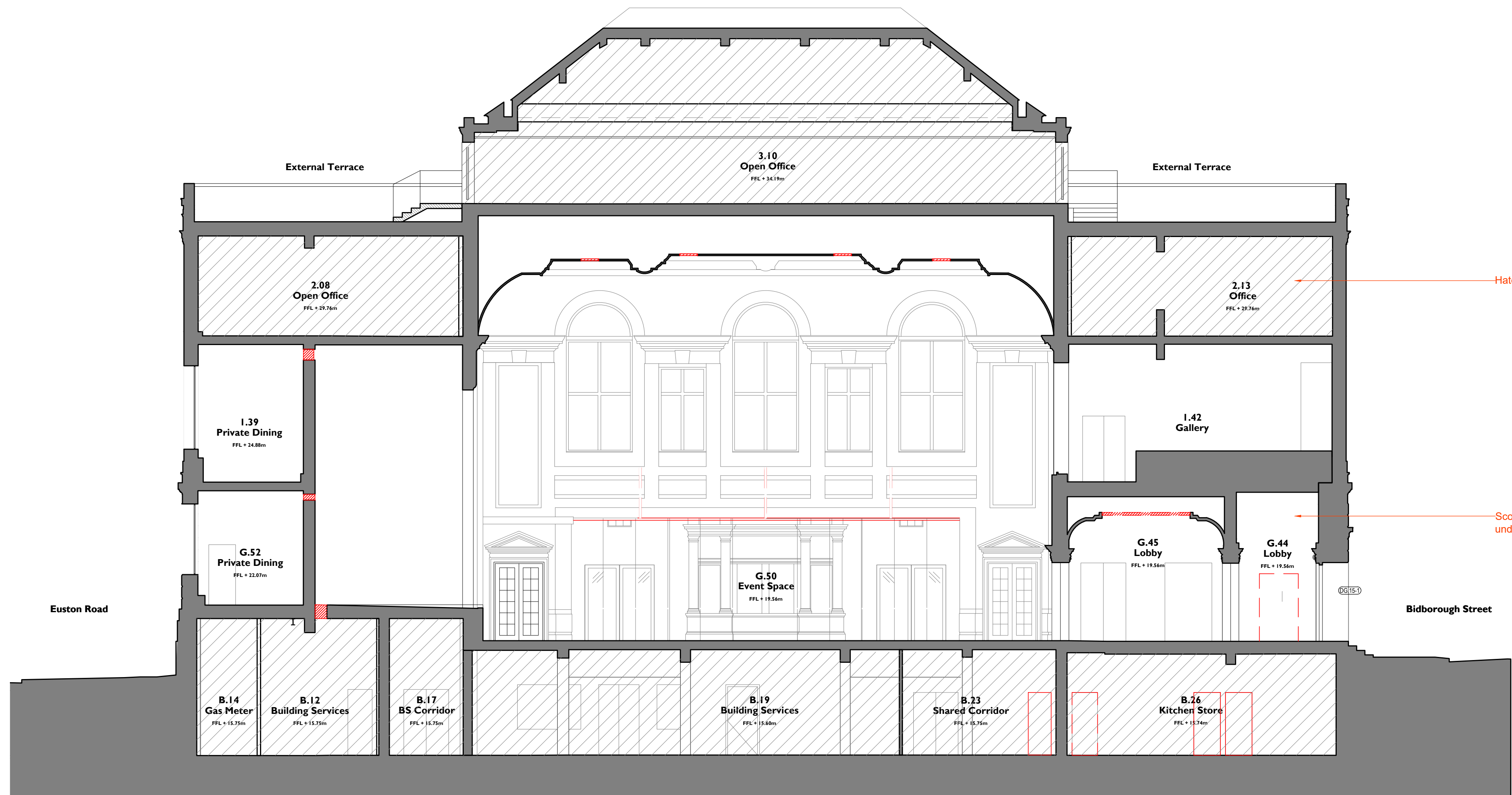
1 SECTION A-A - EXISTING SHOWING DEMOLITION 0020 1:200
