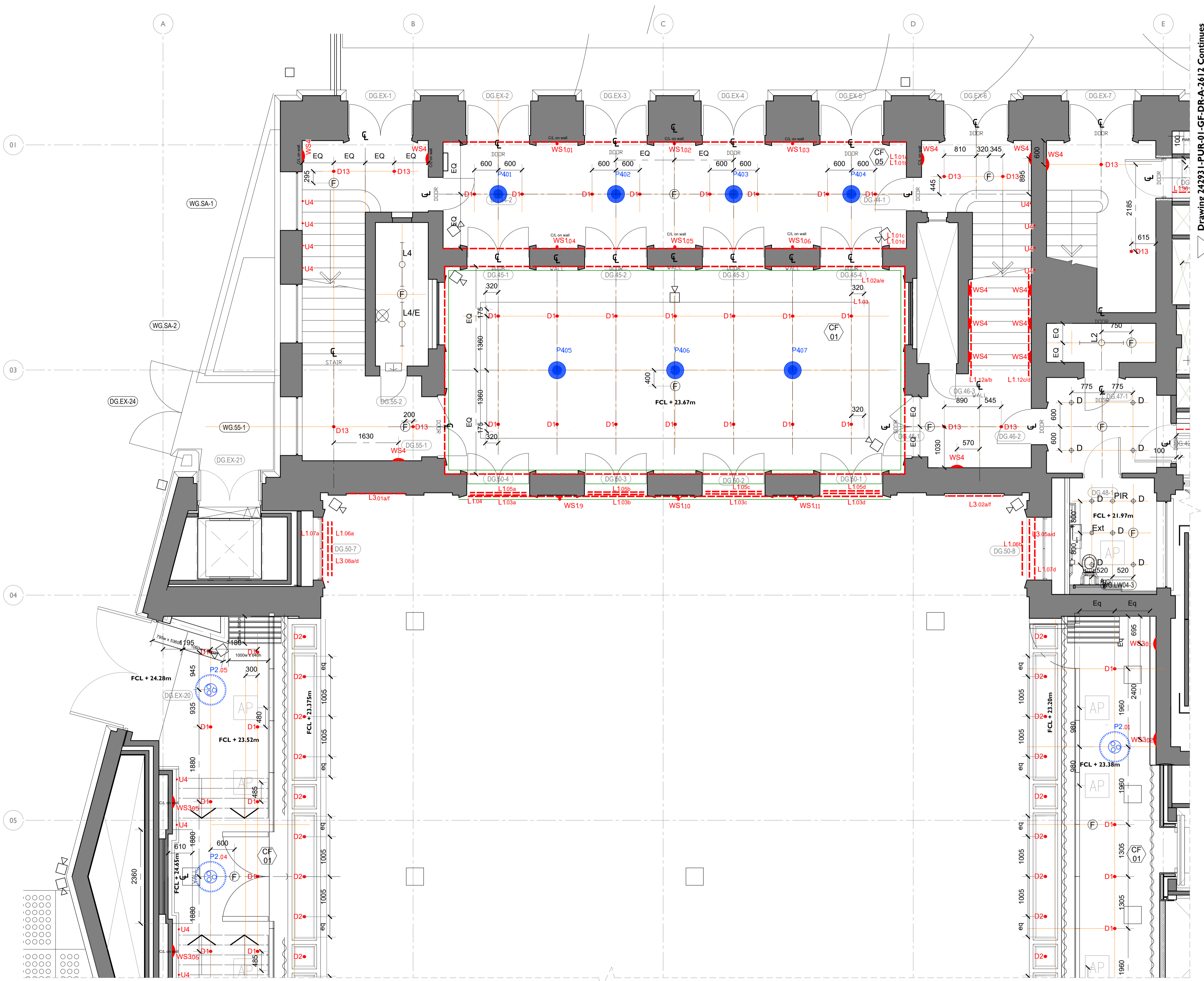
1 PROPOSED RCP - GROUND PLAN 01 2611 1:50 @ A1
