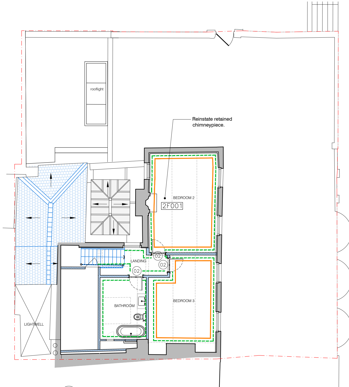
01 Second Floor Plan - 1 : 100 @ A3
