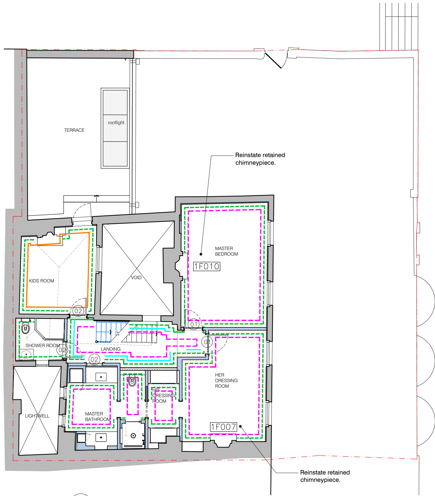
01 First Floor Plan - 1 : 100 @ A3
