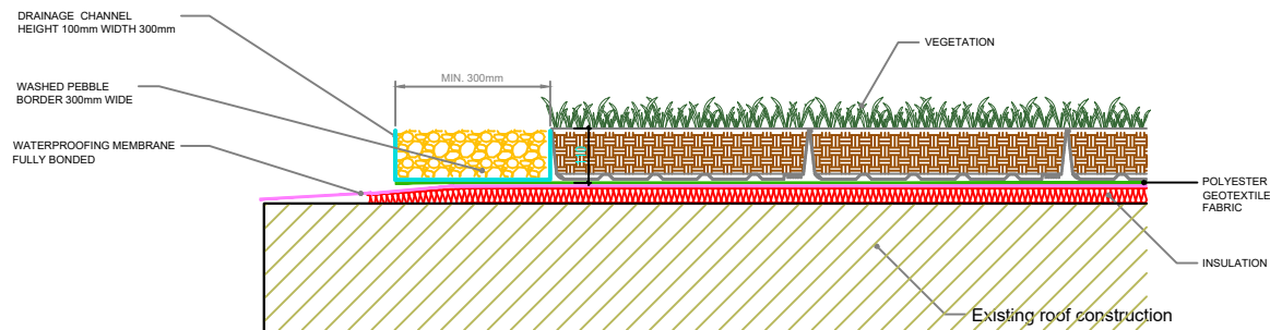
Figure 02 M-TRAY SYSTEM BUILD-UP NTS
