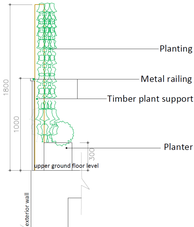
Terrace Screening - section - detail drawing
