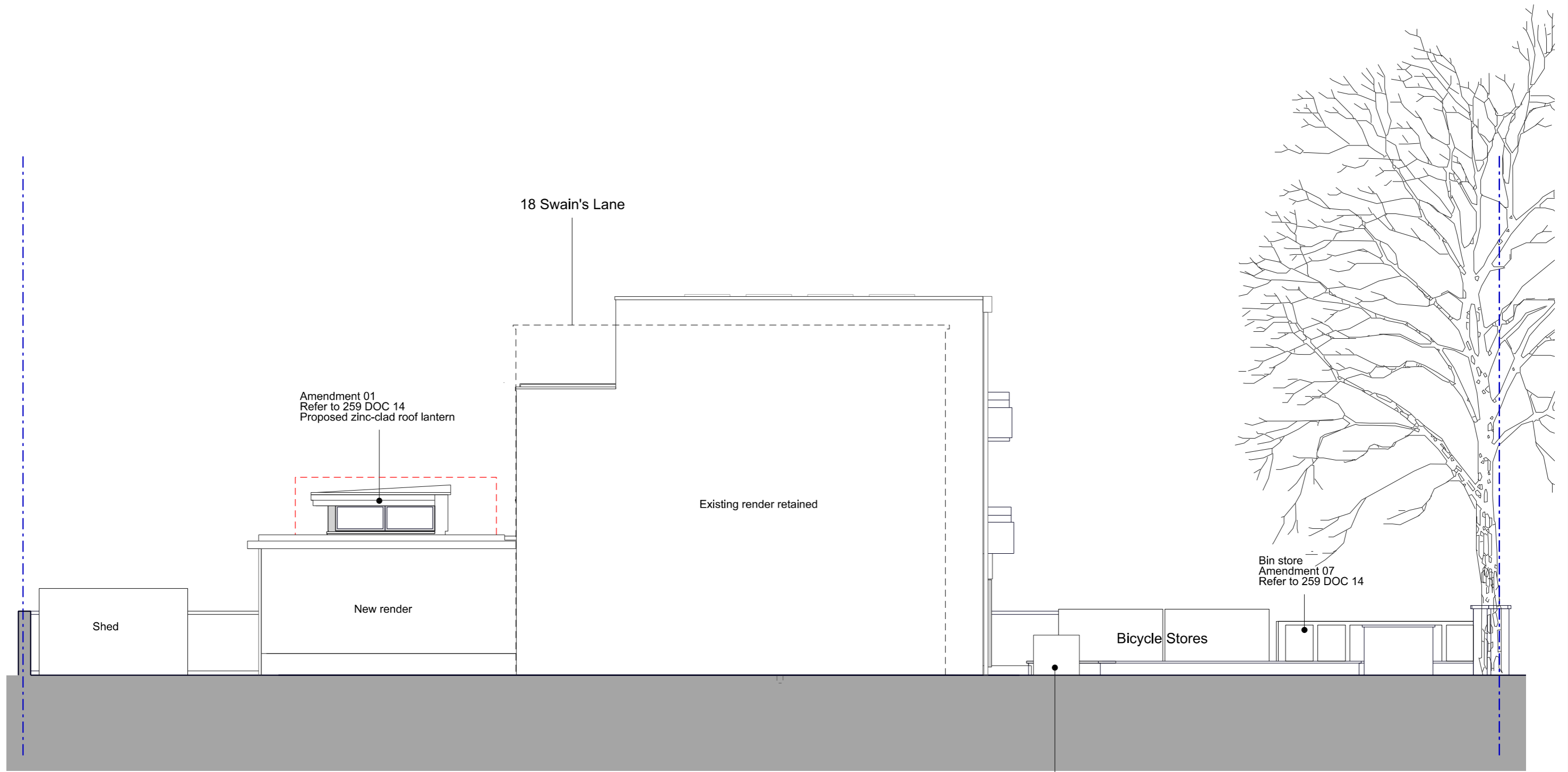
As Proposed East Elevation
