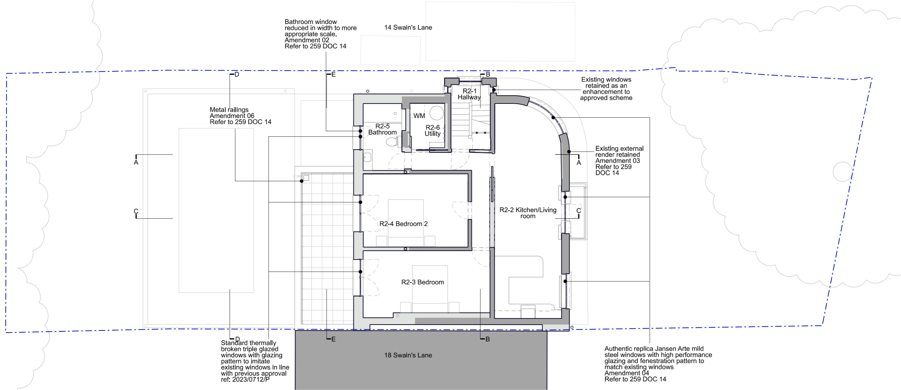
As Proposed Second Floor Plan
