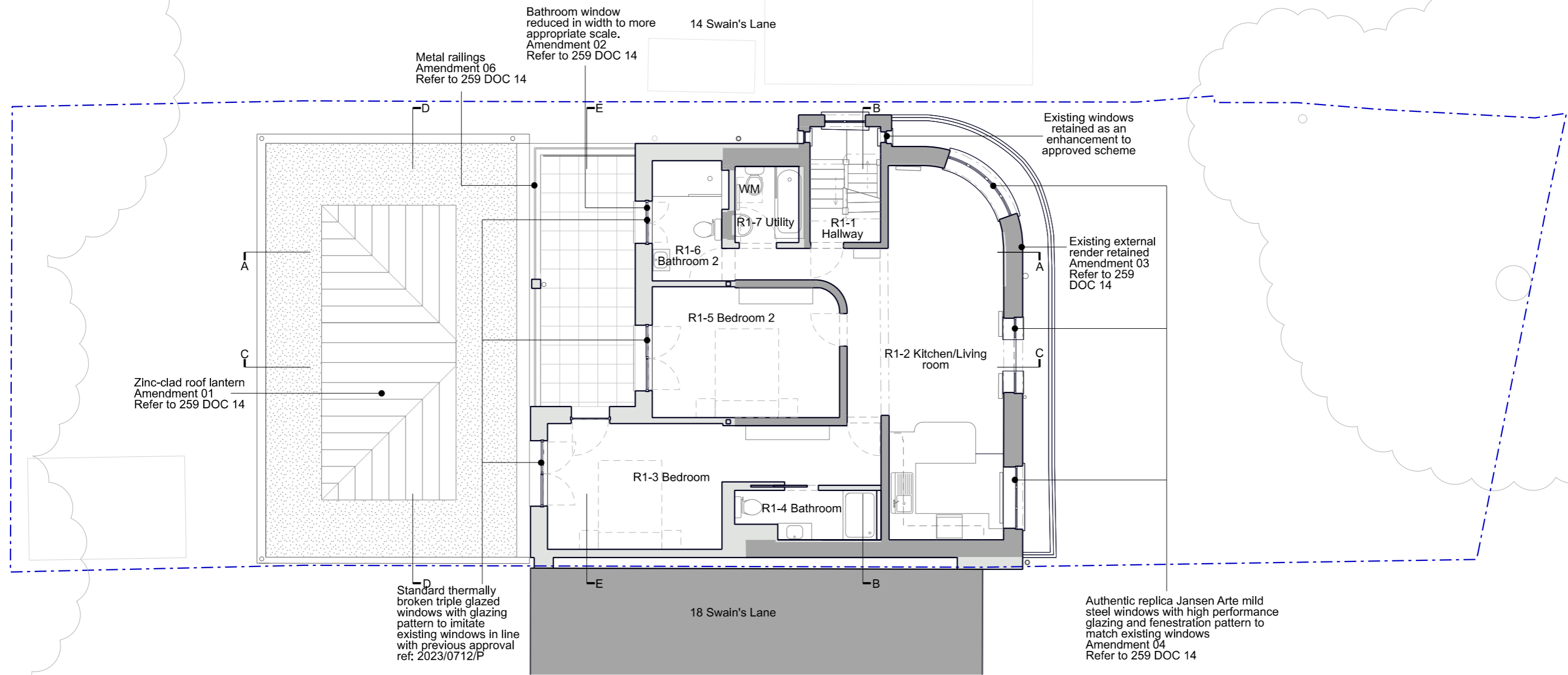
As Proposed First Floor Plan
