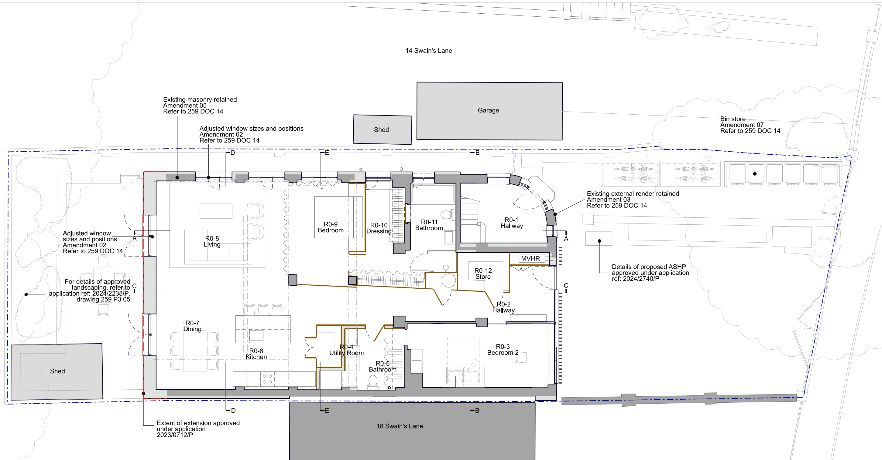
As Proposed Ground Floor Plan
