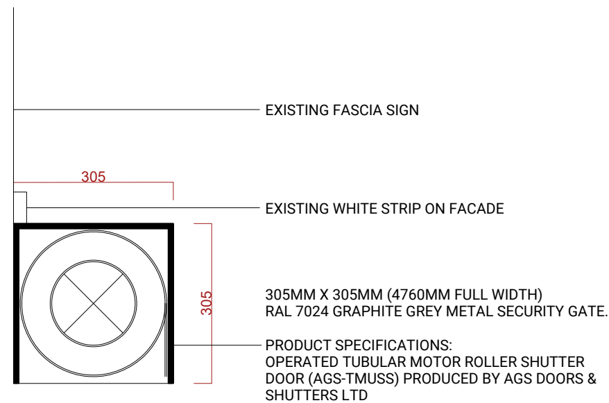
1:10 PROPOSED SIDE SECTION
