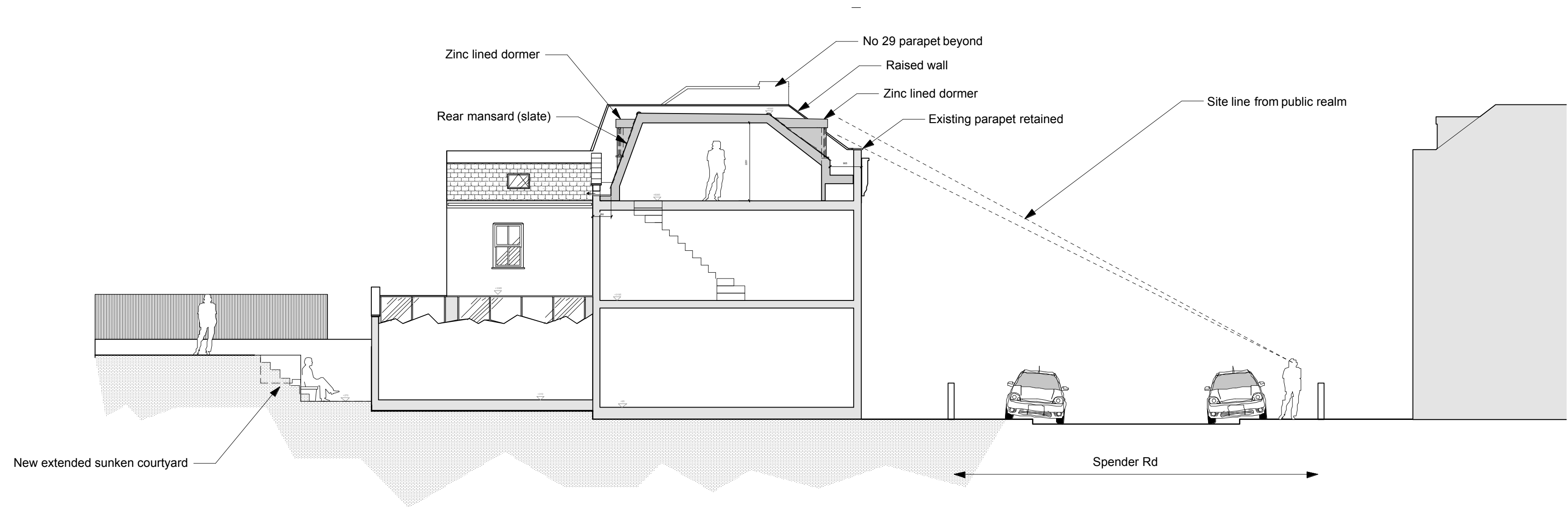
1. PROPOSED LONGITUDINAL SECTION 'ZZ'
