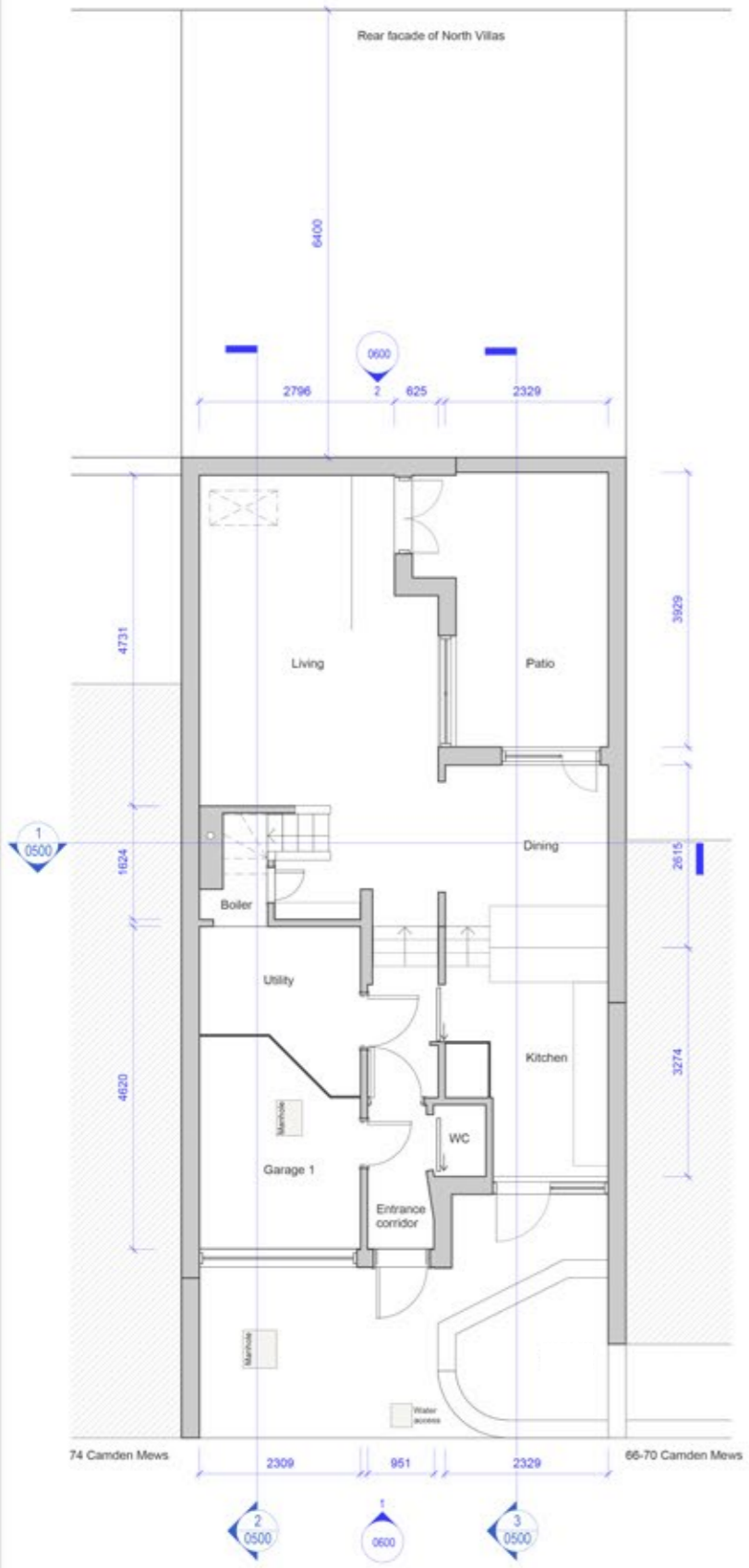
1 Ground Floor Plan 0200 1:50
