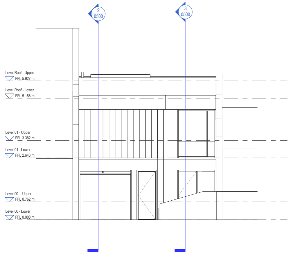
1 Front Elevation 0600 1 : 50
