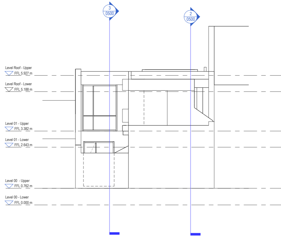
2 Rear Elevation 0600 1 : 50
