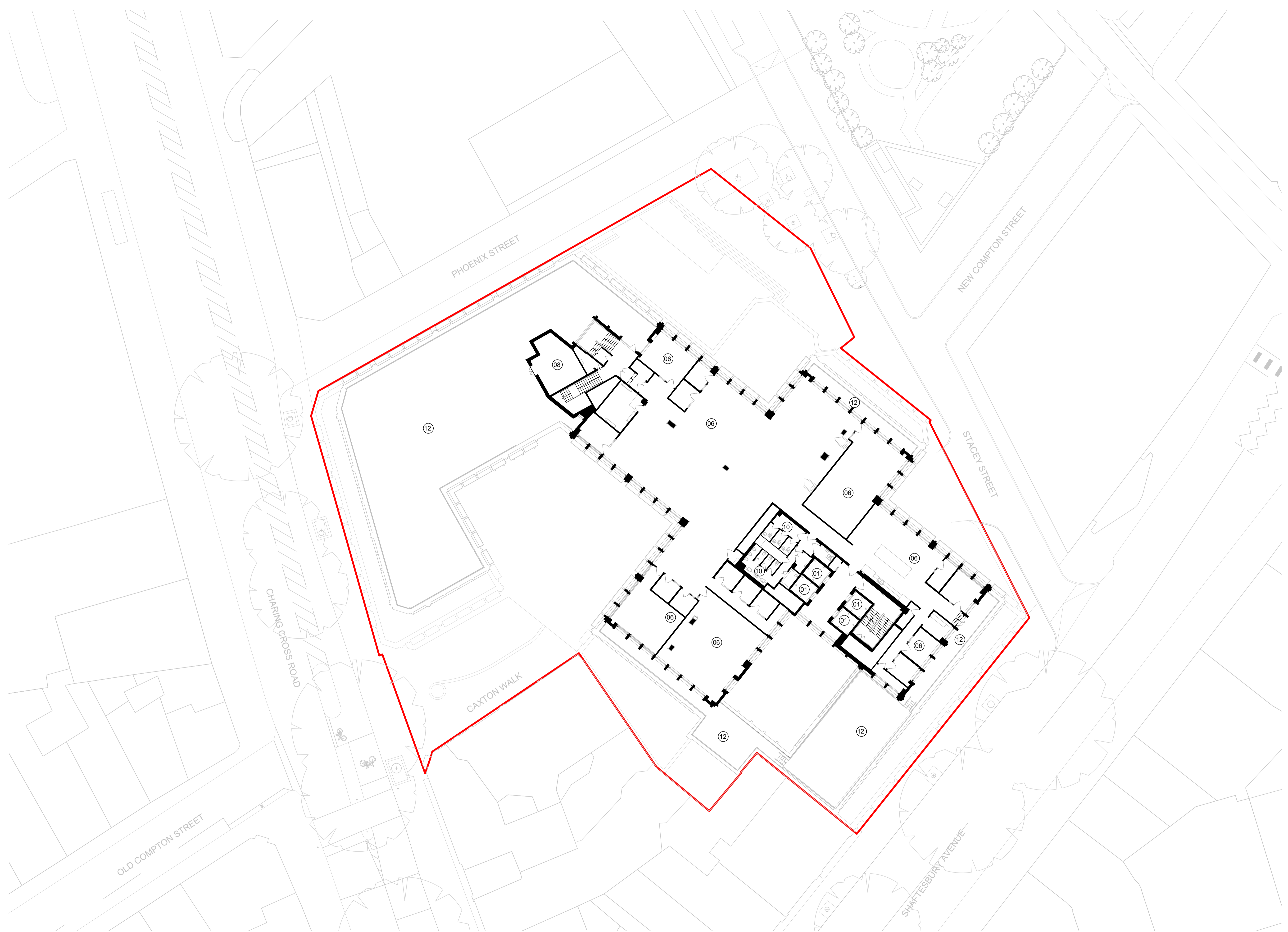
Existing Seventh Floor Plan
