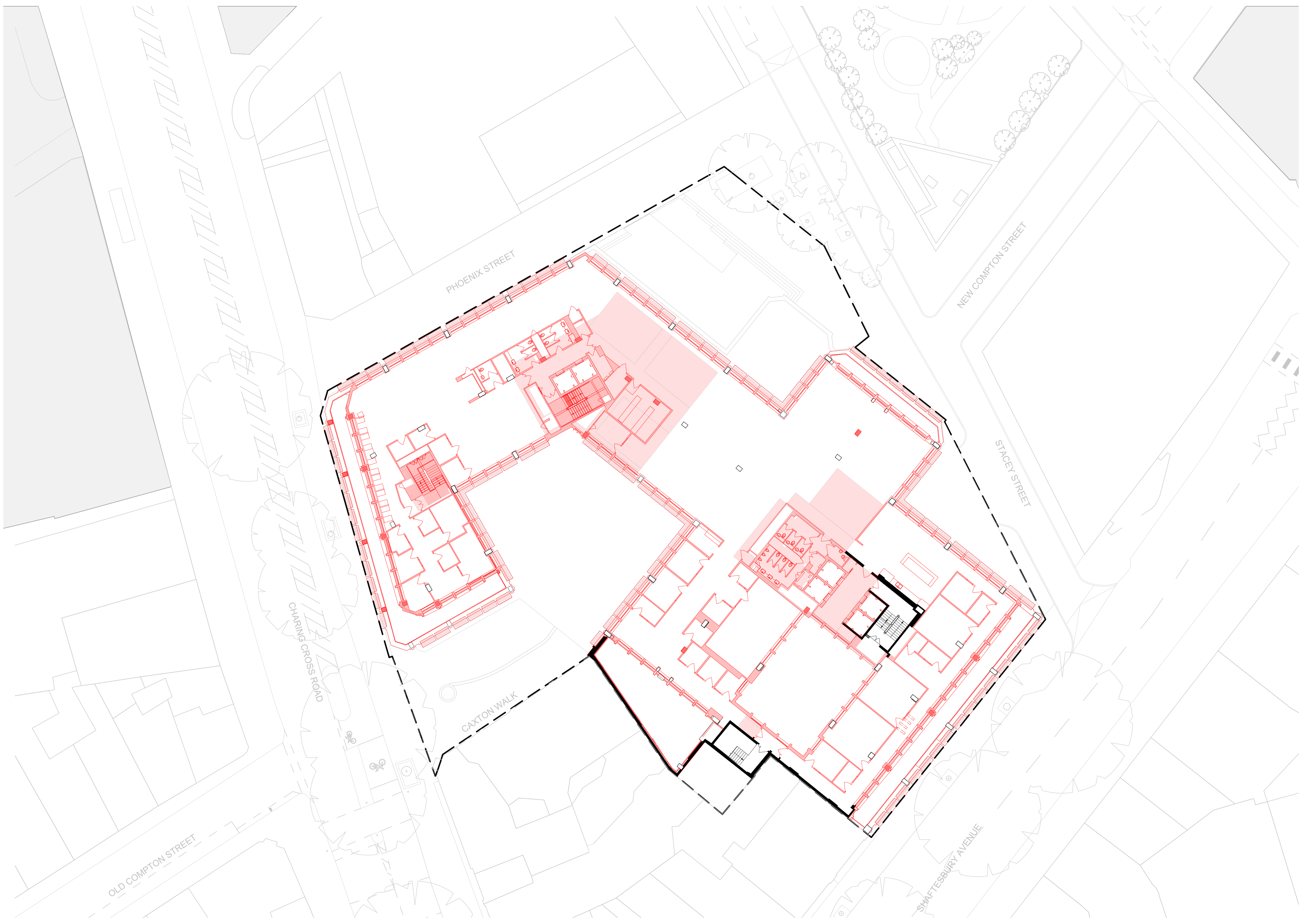
Demolition Sixth Floor Plan
