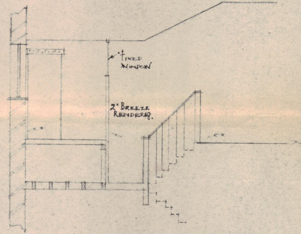
DETAIL A-A. SCALE 1/4" = ONE FOOT.
