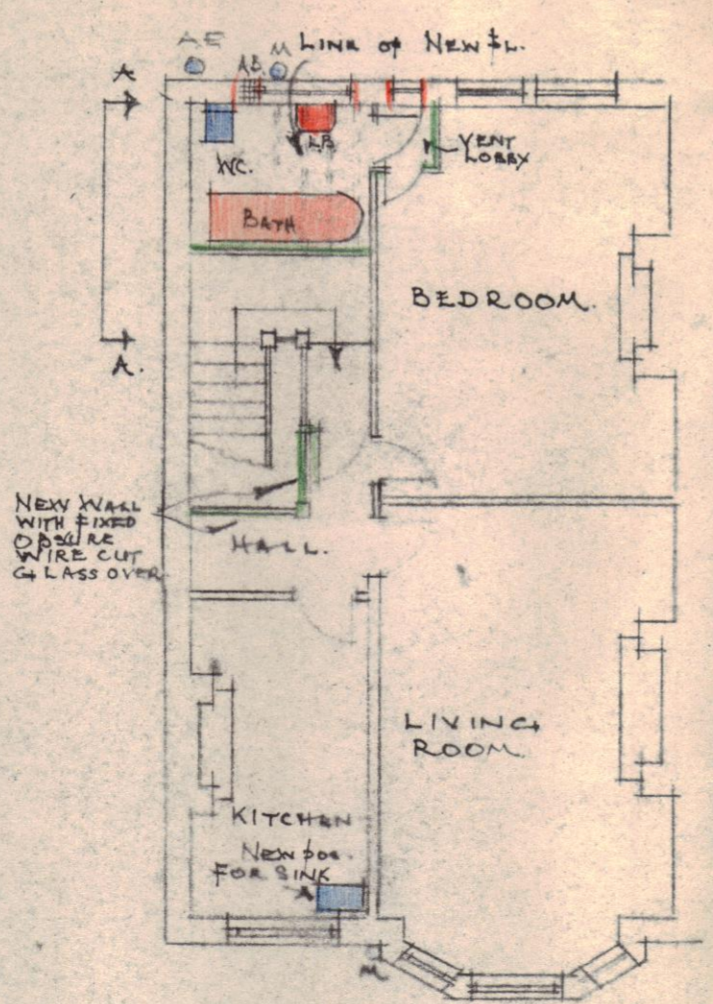
SECOND FLOOR
