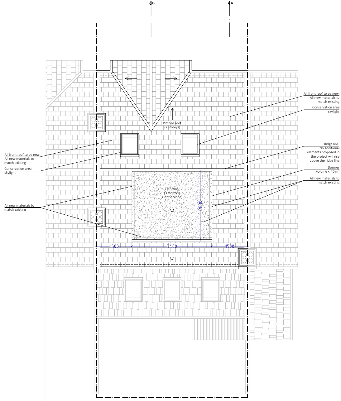
PROPOSED ROOF
