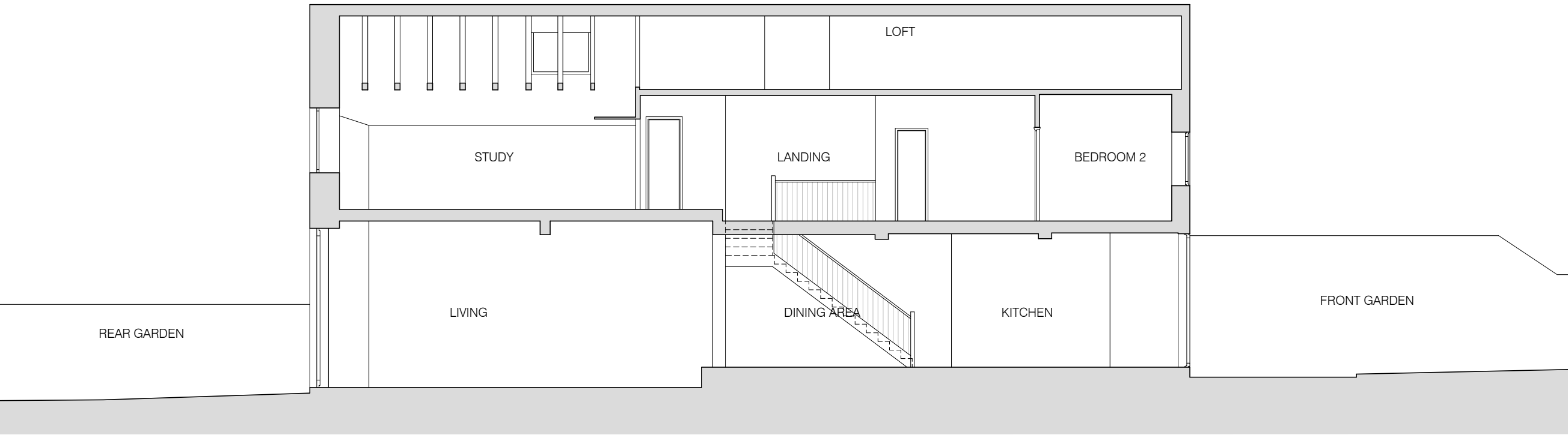
01 EXISTING SECTION A-A scale 1:100
