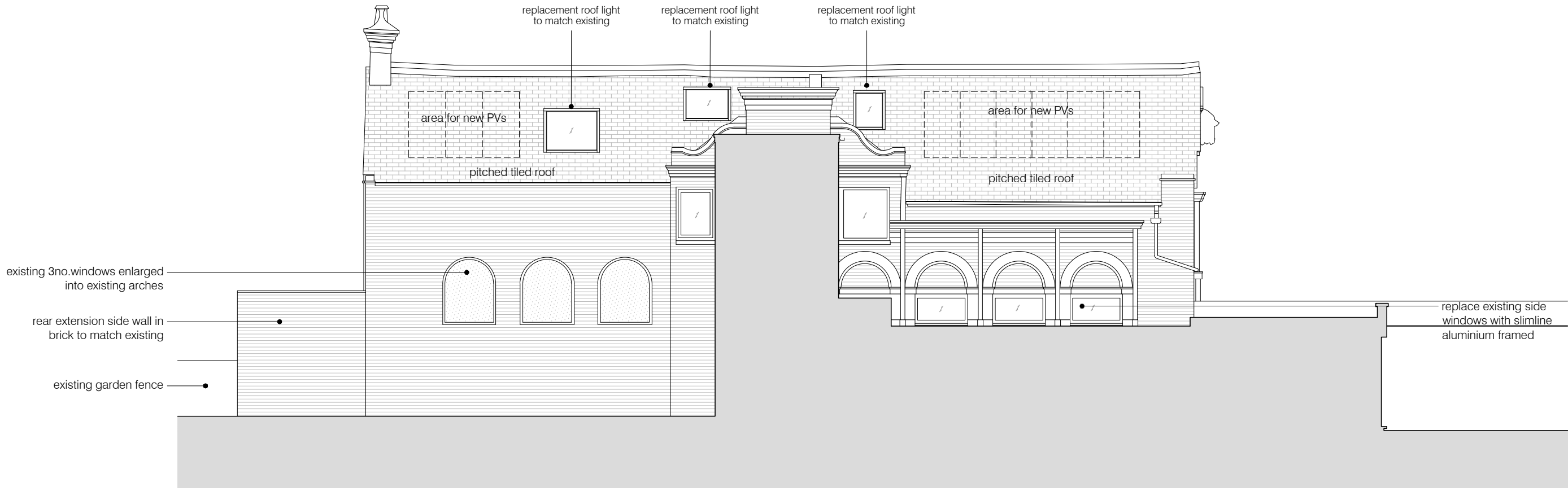
01 PROPOSED SIDE ELEVATION scale 1:100
