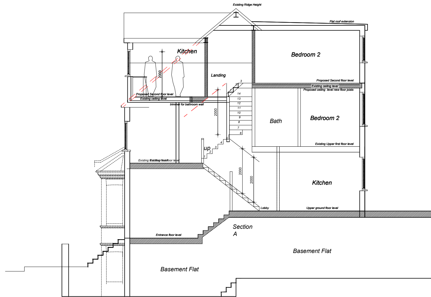
Proposed Section
