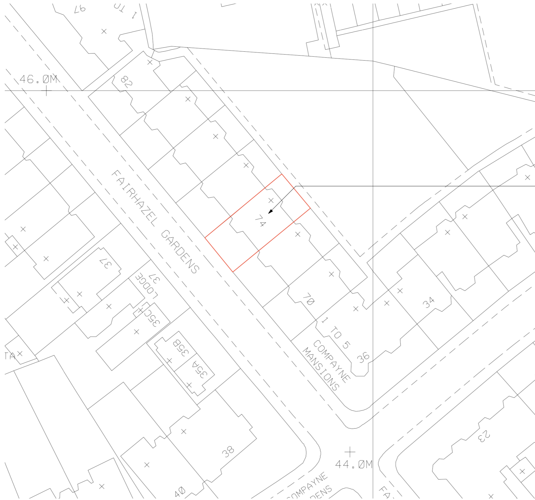
BLOCK PLAN 1:500
