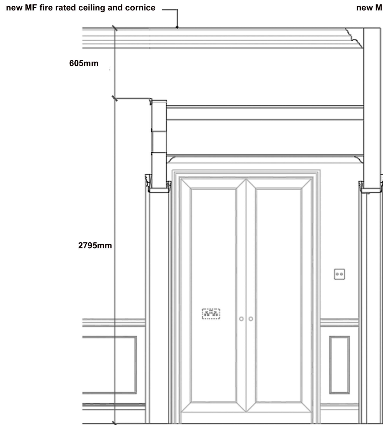
GROUND FLOOR POD ROOM SECTION - NO HISTORIC CEILING
