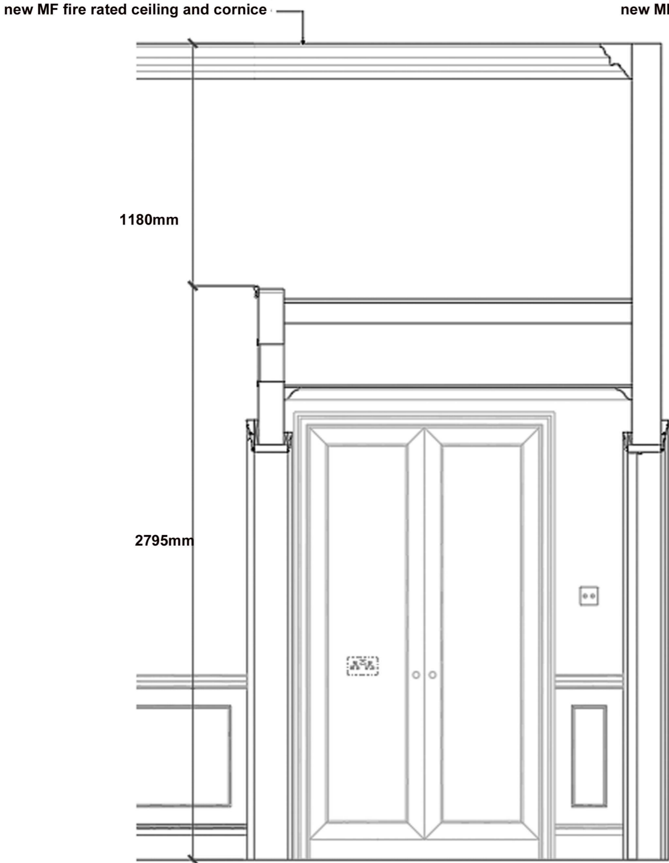
FIRST FLOOR POD ROOM SECTION - NO HISTORIC CEILING
