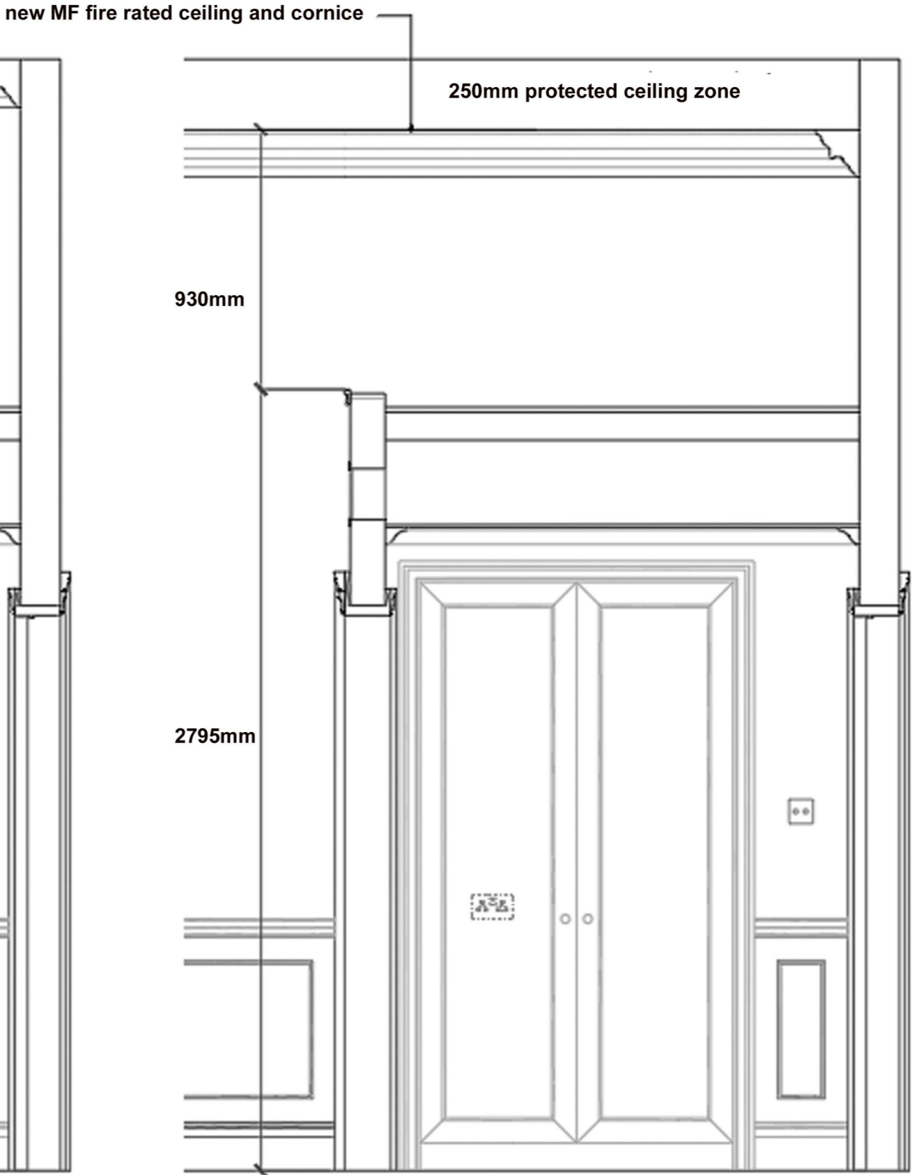
FIRST FLOOR POD ROOM SECTION - HISTORIC CEILING RETAINED
