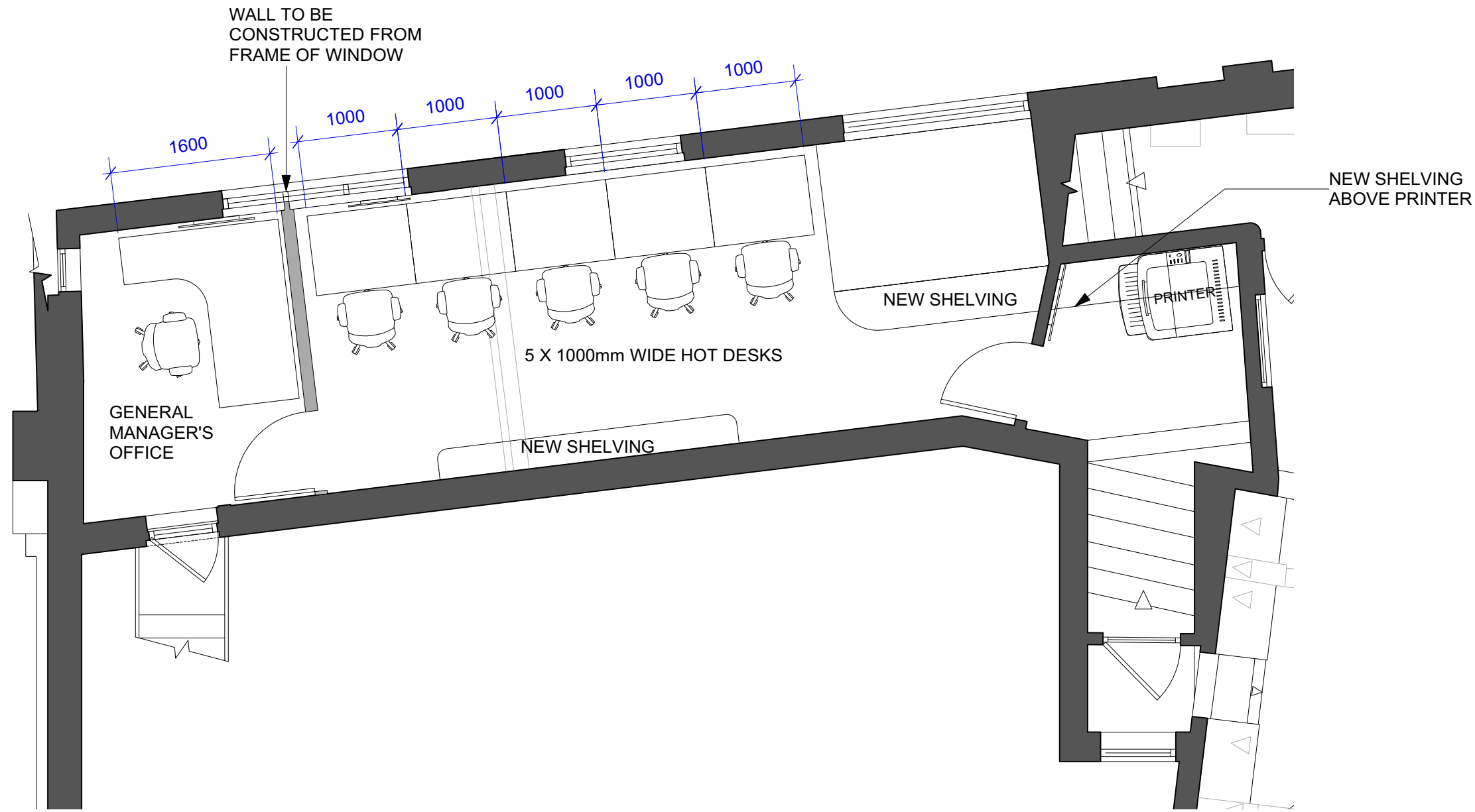
1 Office Plan As Proposed Scale: 1:50 @ A3
