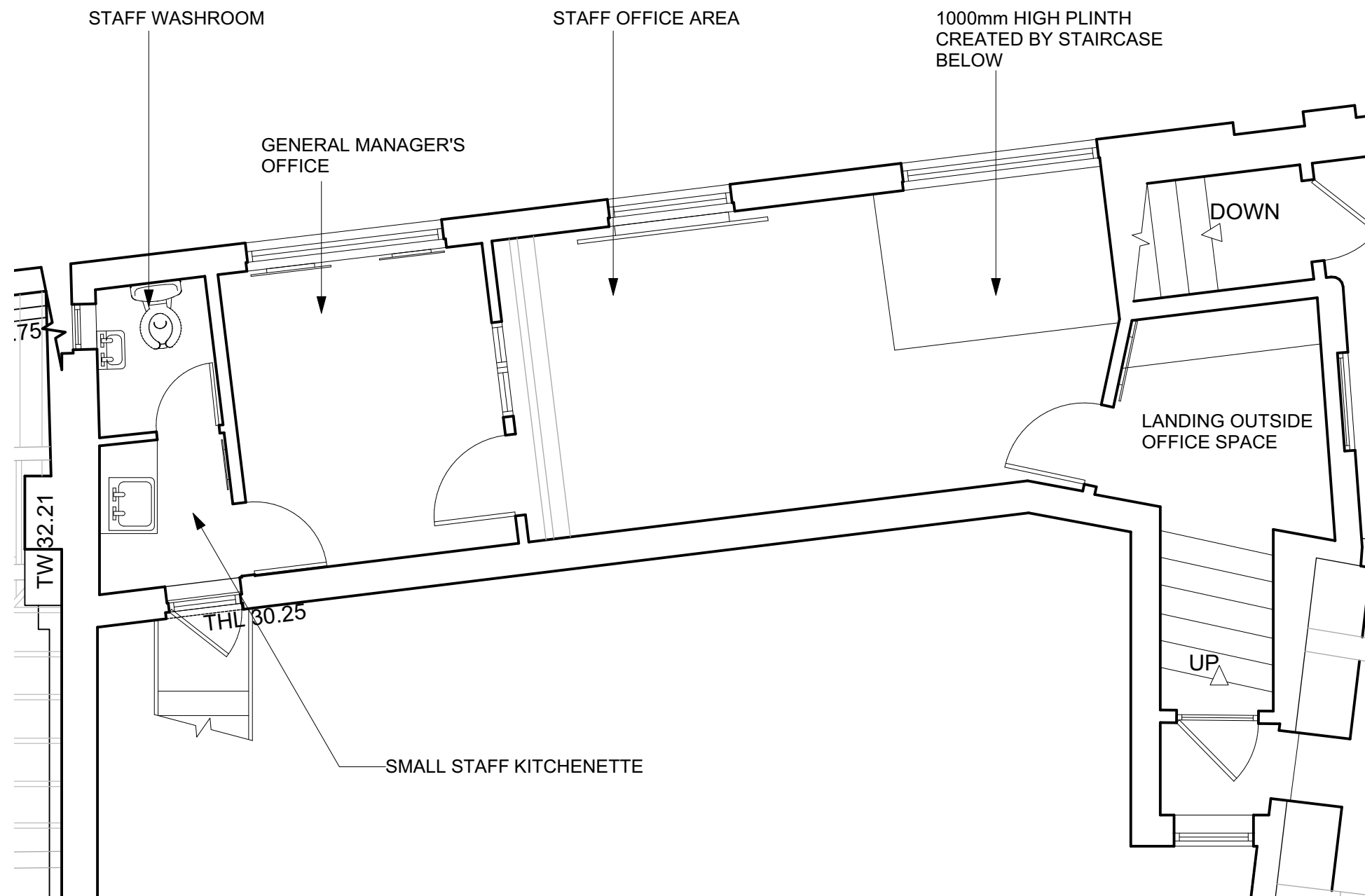
1 Office Plan As Existing Scale: 1:50 @ A3
