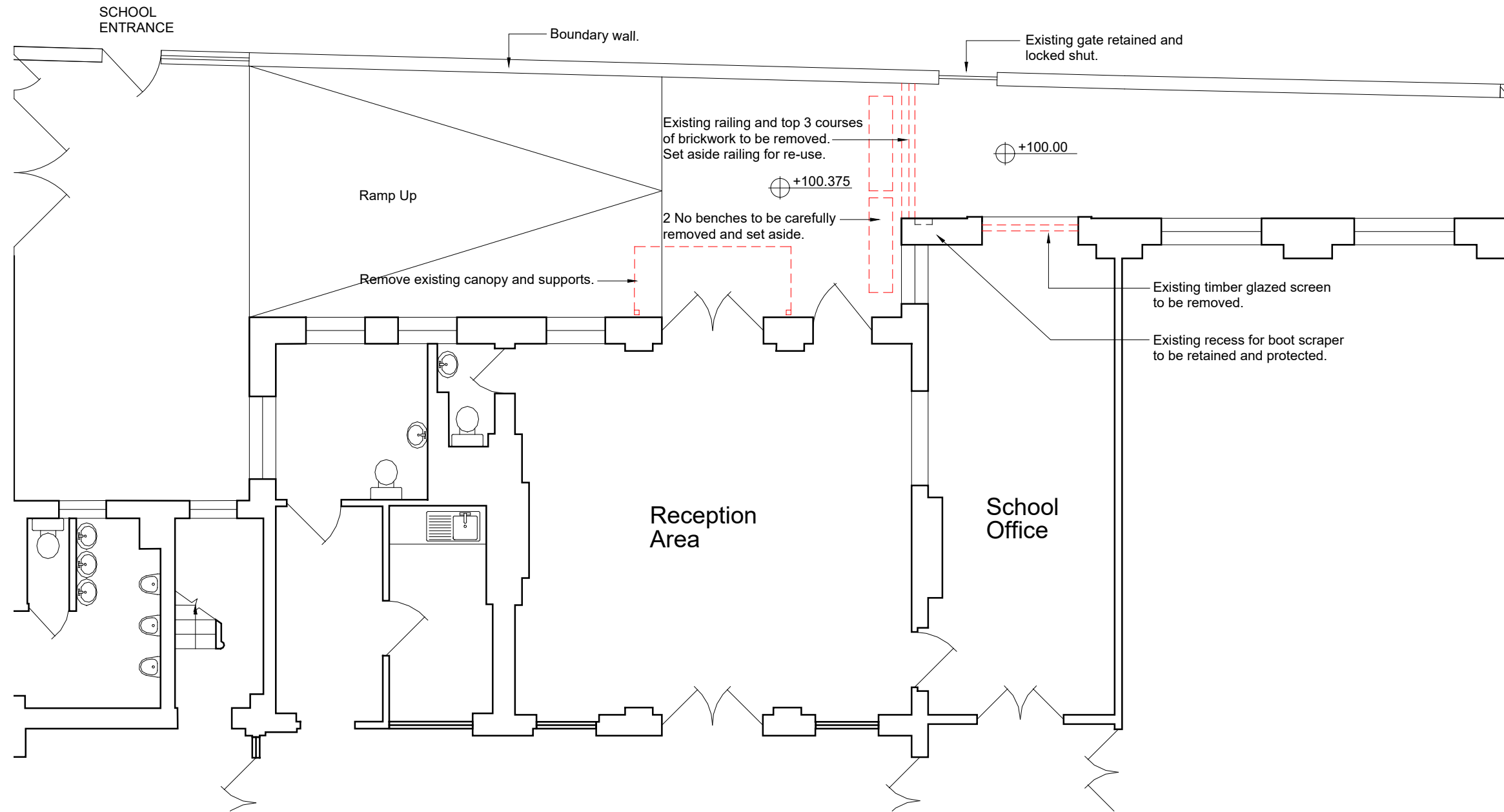
1 Existing Ground Floor Plan A03 Scale 1:50
