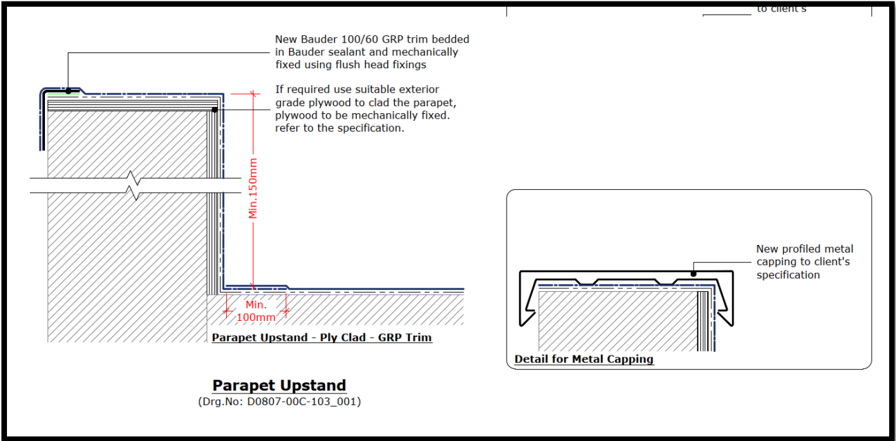
Section of Works to Roof B-F (Dwg No. D0807-00C-100_001) submitted June 2024
