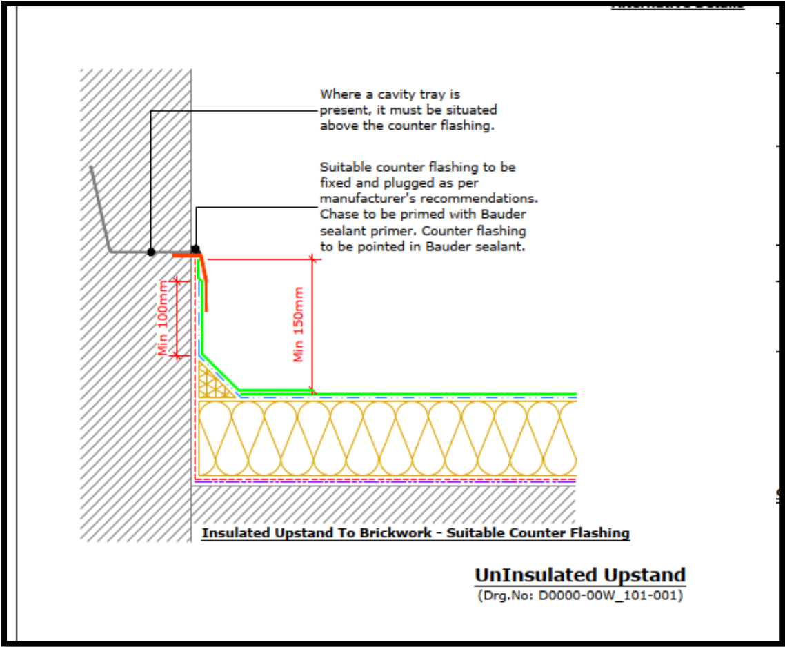
Section of Works to Roof A (Dwg No. D0000-00W_100-001) submitted June 2024
