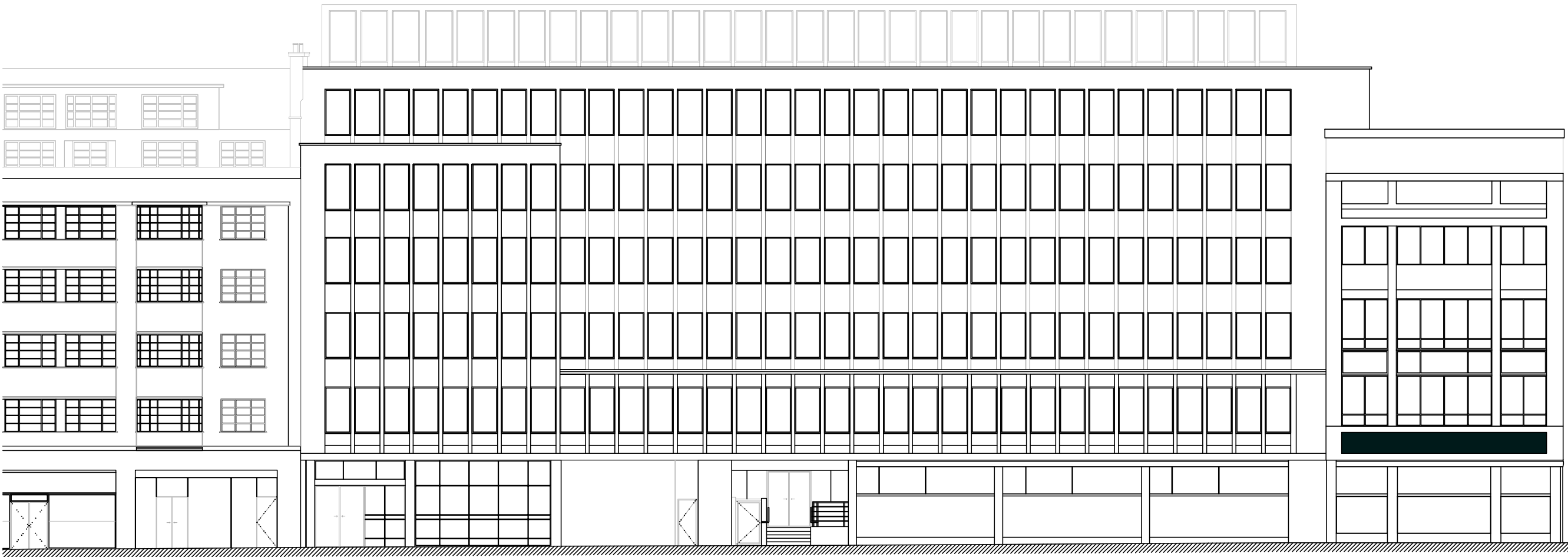
Existing Torrington Place Elevation Scale 1:200
