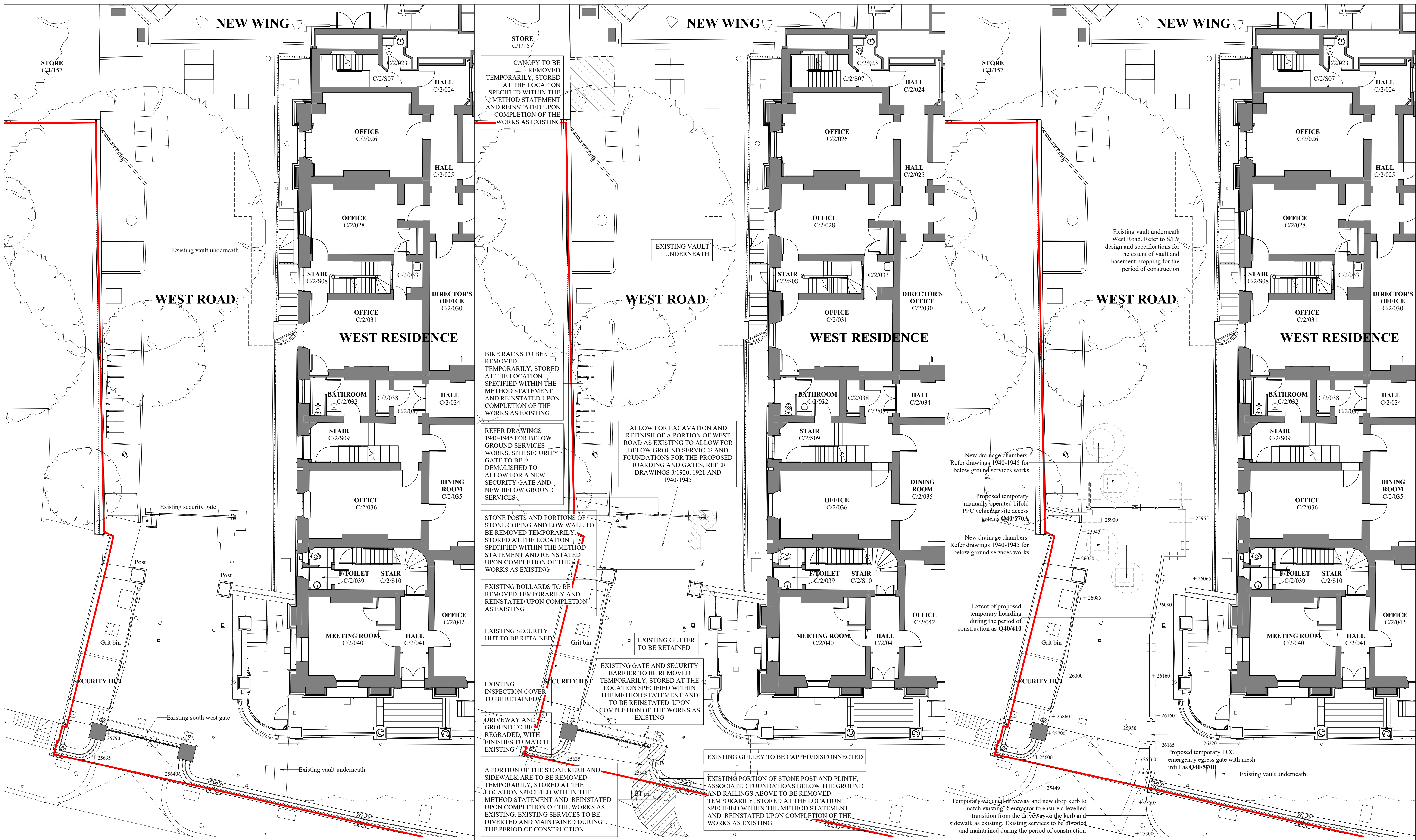
3 Construction Access 1 : 100
