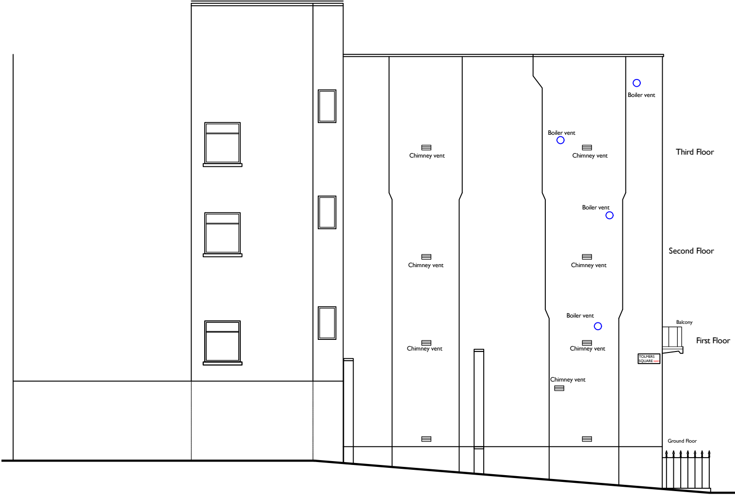
Tolmers Square Elevation C
