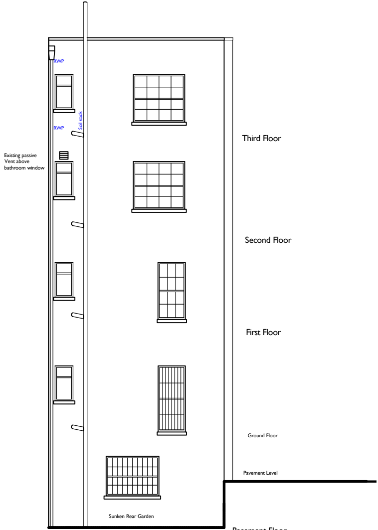
Part Rear Elevation D
