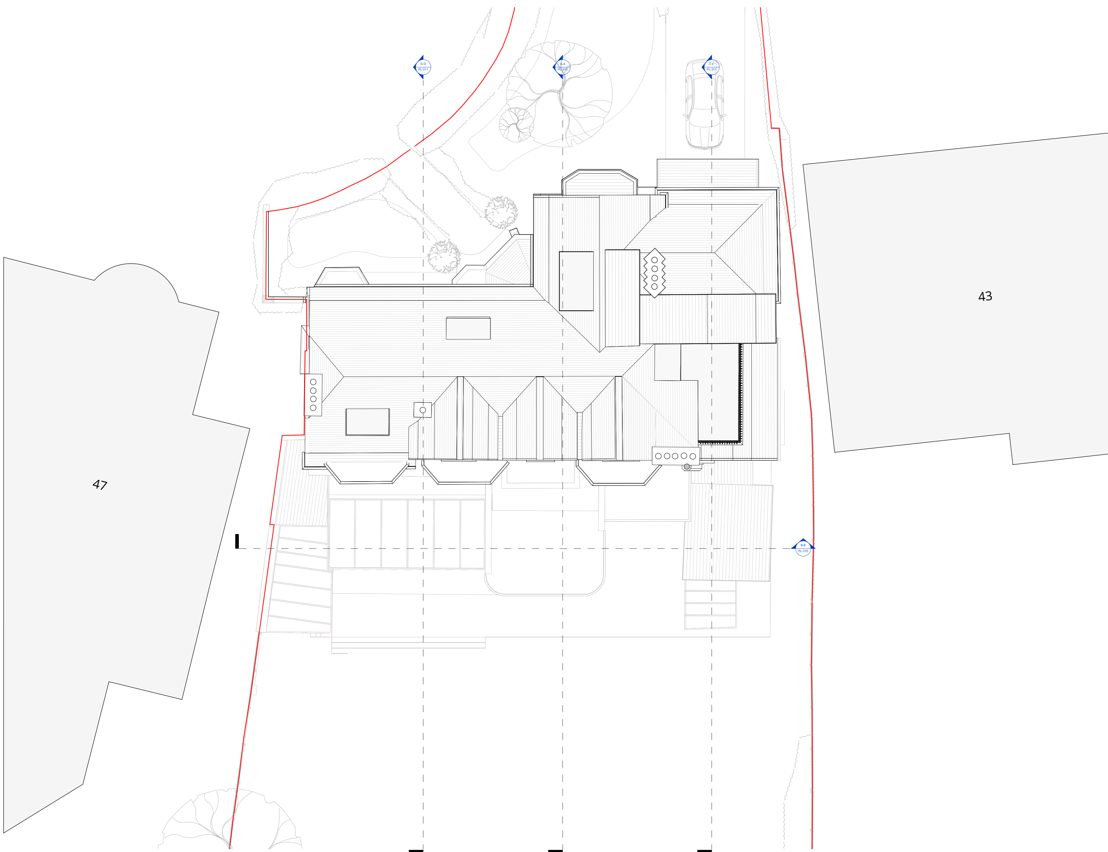
Proposed Roof 1:100
