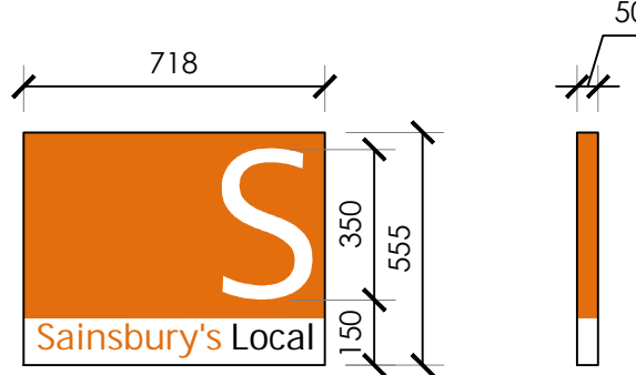
PROPOSED BUS STOP SIGN SCALE (1:20 @ A1)
