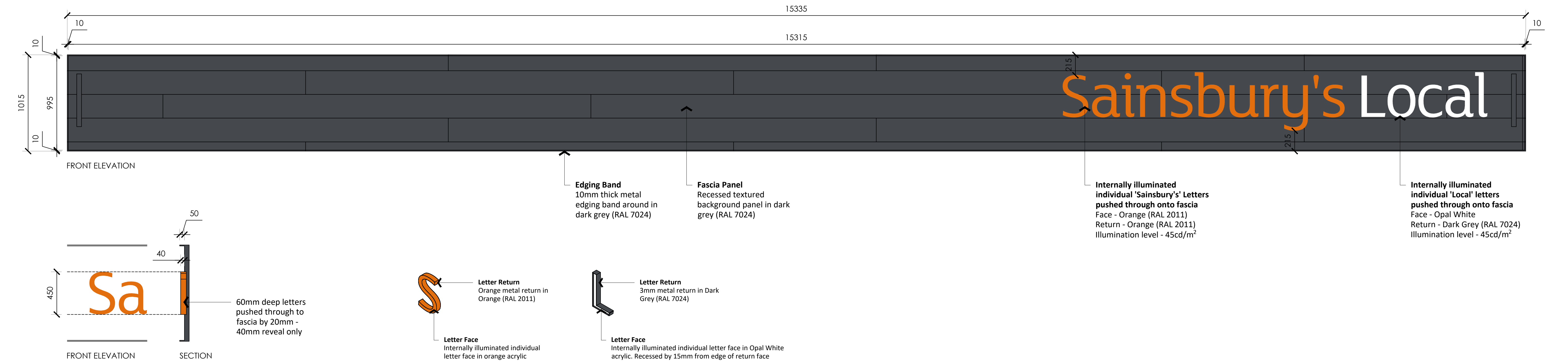
PROPOSED FASCIA SIGN LETTERING DETAILS SCALE (1:20 @ A1)
