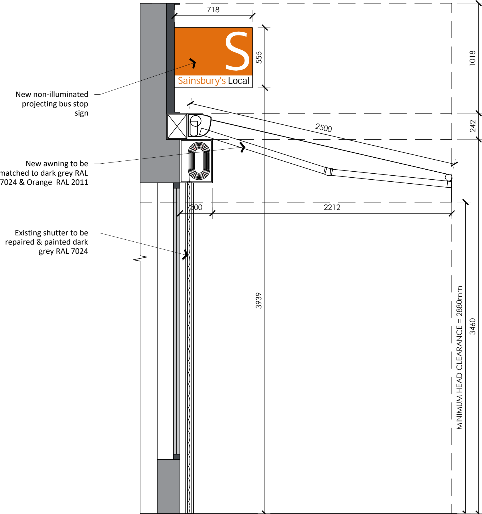
PROPOSED SHOPFRONT SECTION SCALE (1:20 @ A1)
