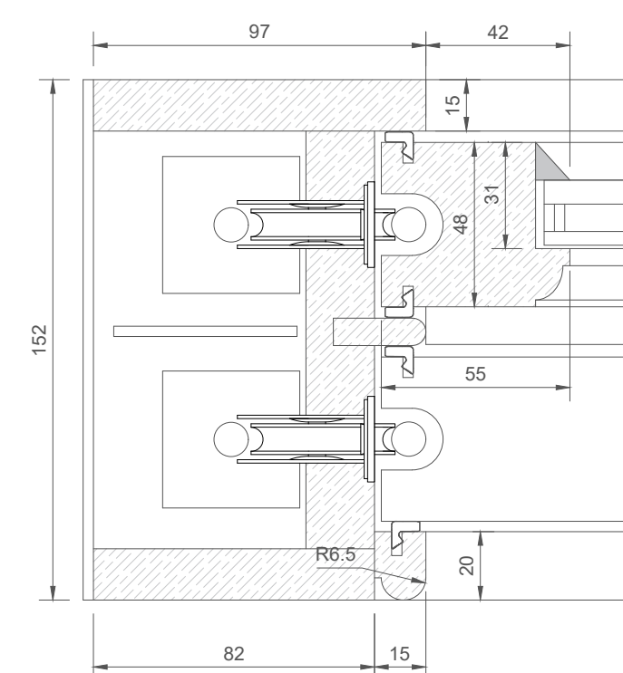
Width Section B-B
