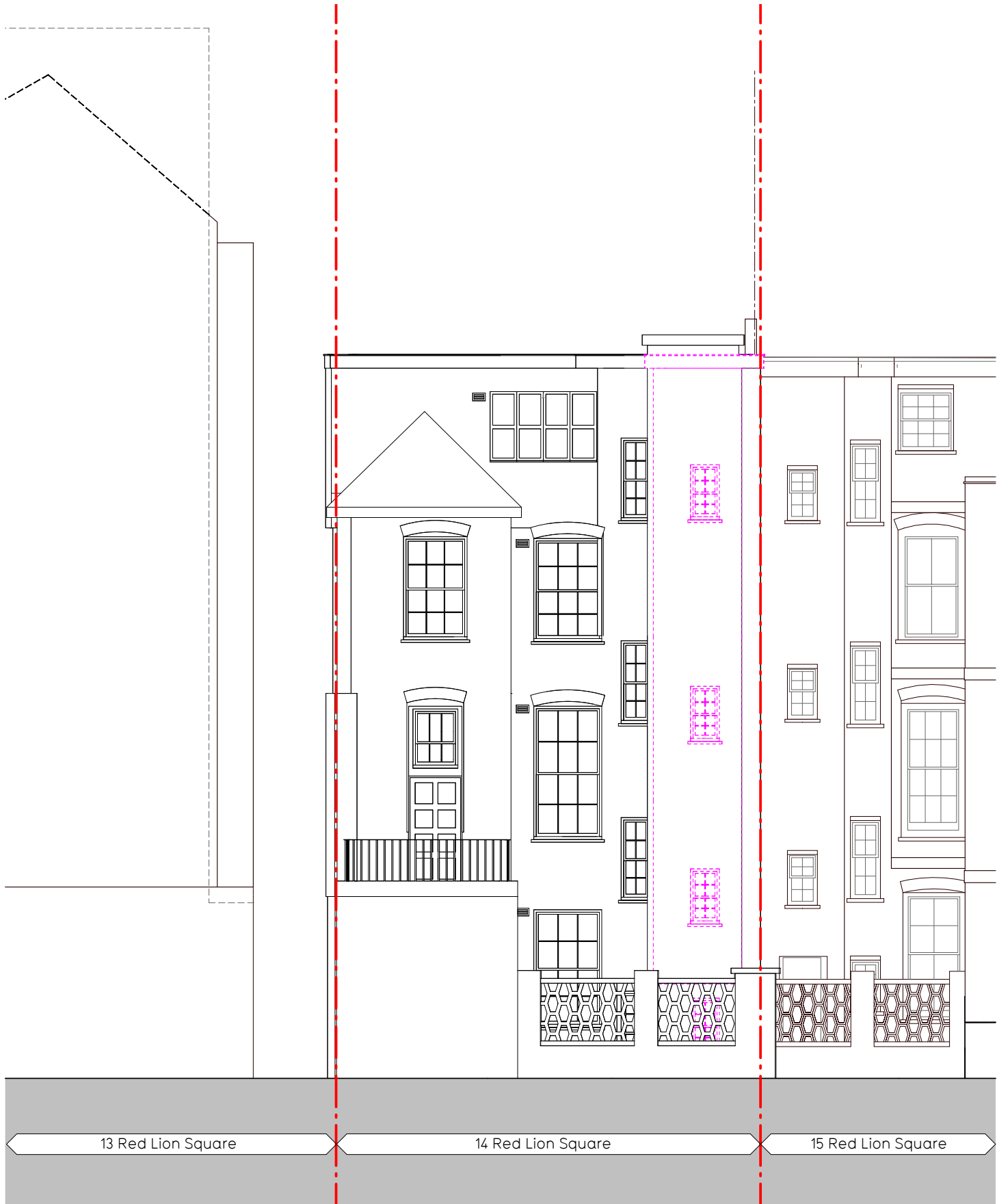
1 Rear elevation - Demolition extent 301 1:100
